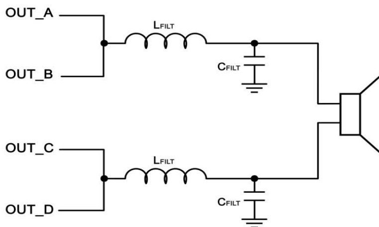
FIG 58. Pre-Filter PBTL
