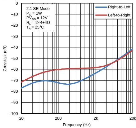
Figure 15. Crosstalk vs Frequency
