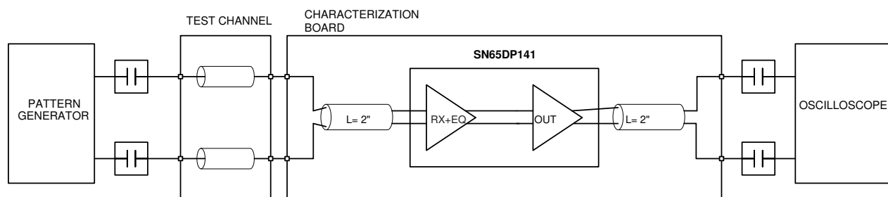
FIG 7-6. Receive Side Performance Test Circuit
