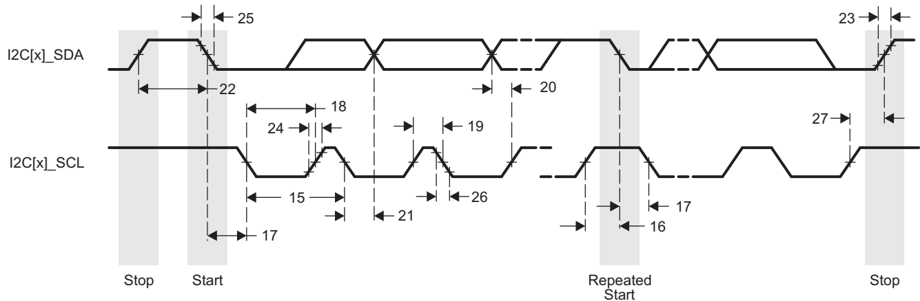
図 7-69. I 2 C Transmit Timing
