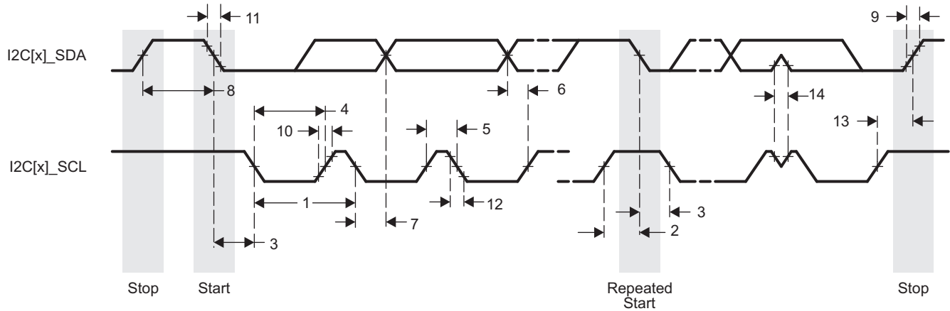
図 7-68. I 2 C Receive Timing
