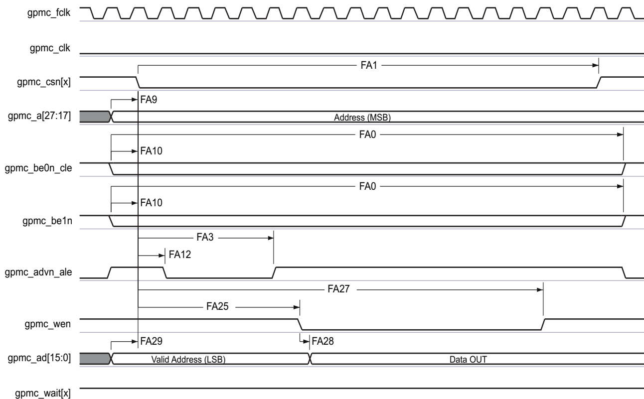
7-27. GPMC and Multiplexed NOR Flash—Asynchronous Write—Single Word
