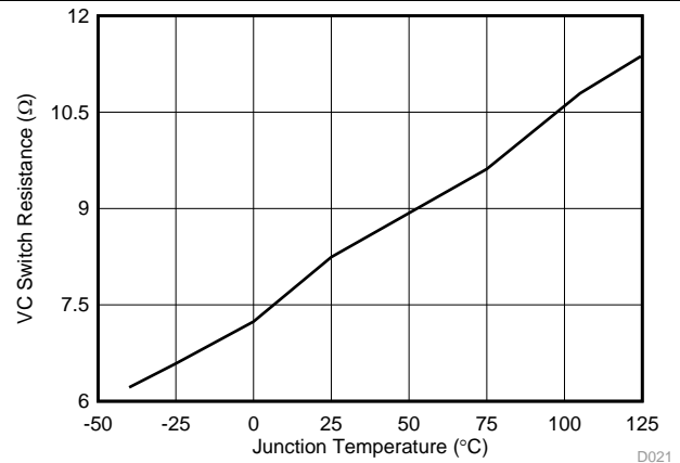
Figure 20. VC Switch Resistance vs Temperature
