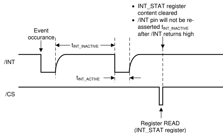
FIG 8-7. Dynamic \overline{\text{INT}} Assertion Scheme With INT_STAT Register Read During t_{\text{INT\_INACTIVE}}
