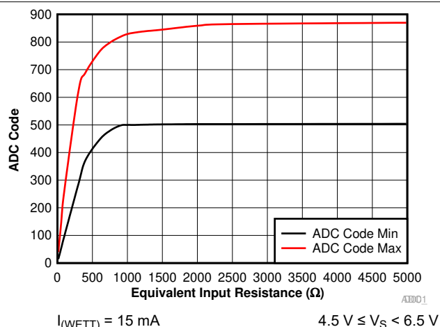
6-10. ADC Code vs. Equivalent Input Resistance
