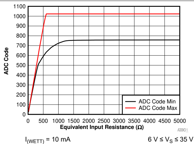
6-9. ADC Code vs. Equivalent Input Resistance
