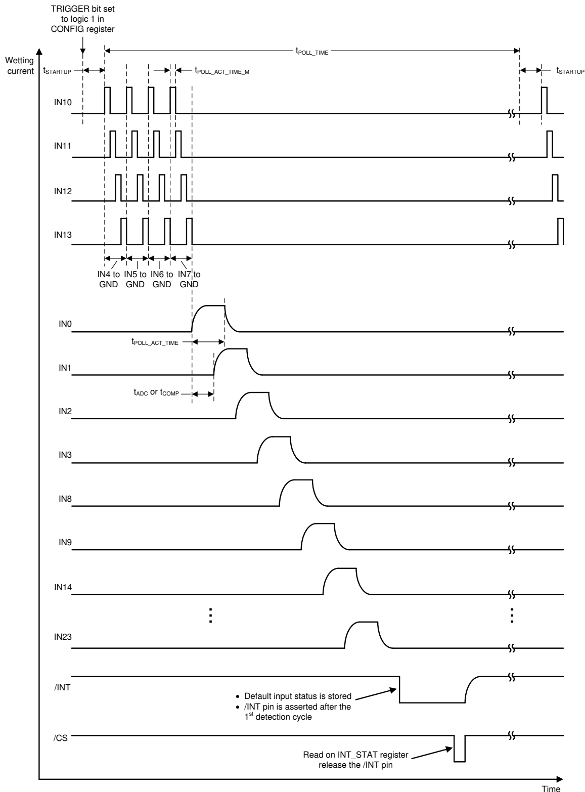
8-17. Polling Scheme for 4×4 Matrix Inputs
