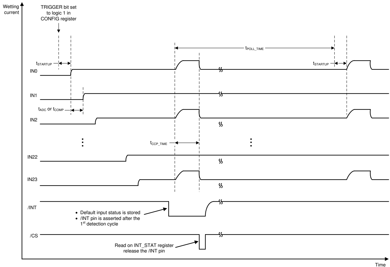
8-19. Continue Mode With CCP Enabled
