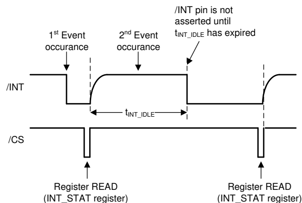
FIG 8-8. \overline{\text{INT}} Assertion Scheme With t_{\text{INT\_IDLE}}
