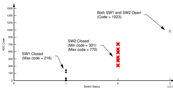
FIG 9-7. Measured ADC Code Distribution for the 3 Switch States
