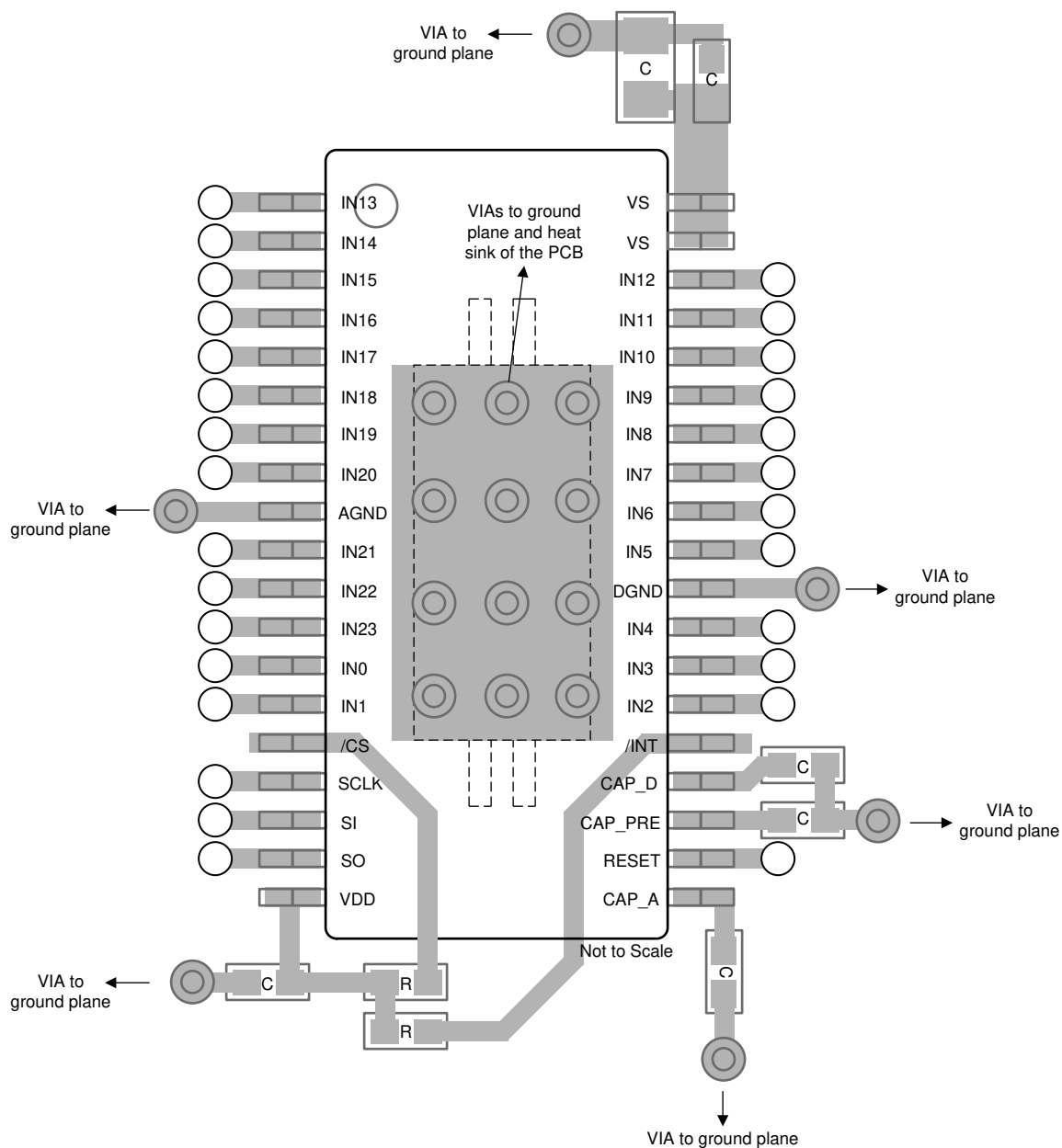
☒ 11-1. Example Layout
