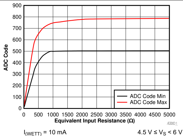
6-8. ADC Code vs. Equivalent Input Resistance
