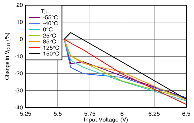
7-54. Line Regulation vs V_{IN}
