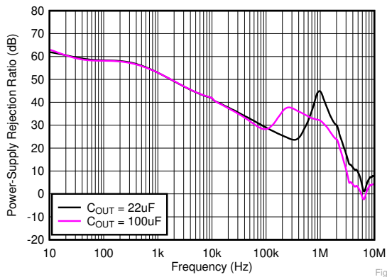
Fig 7-7. PSRR vs Frequency and C_{OUT}
