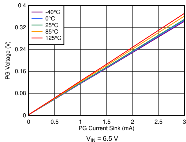
FIG 7-41. PG Voltage vs PG Current Sink
