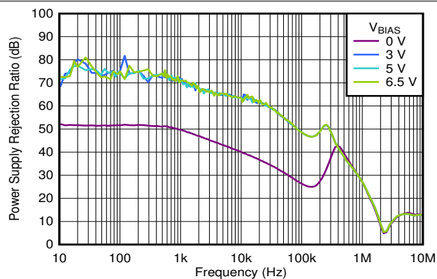
FIG 7-44. PSRR vs Frequency and V_{BIAS}
