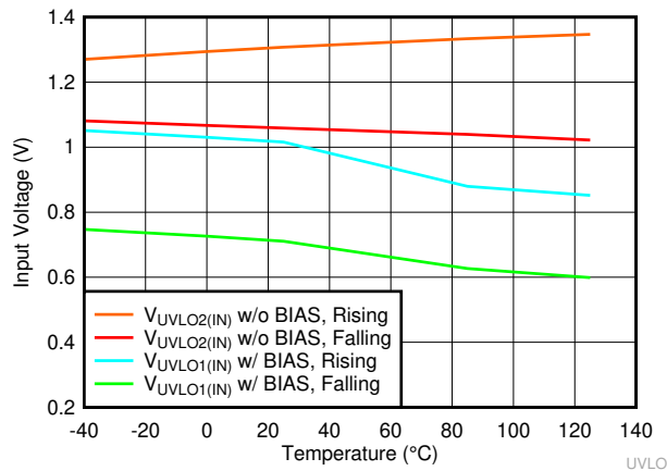
FIG 7-37. V_{IN} UVLO vs Temperature
