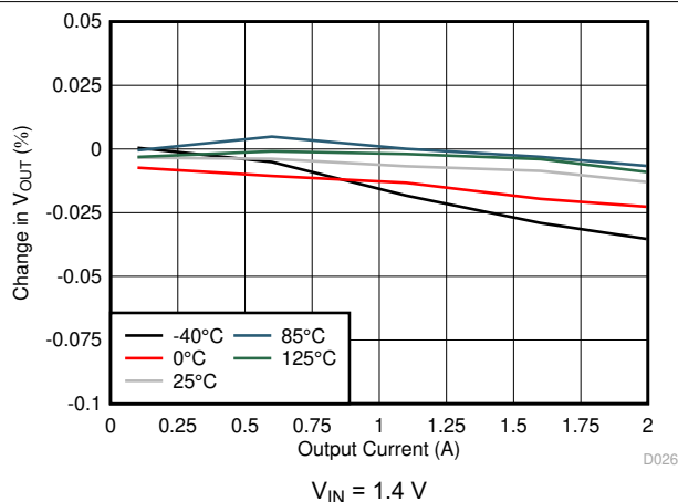
FIG 7-26. Load Regulation
