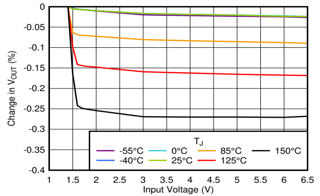
7-54. Line Regulation vs V_{IN}
