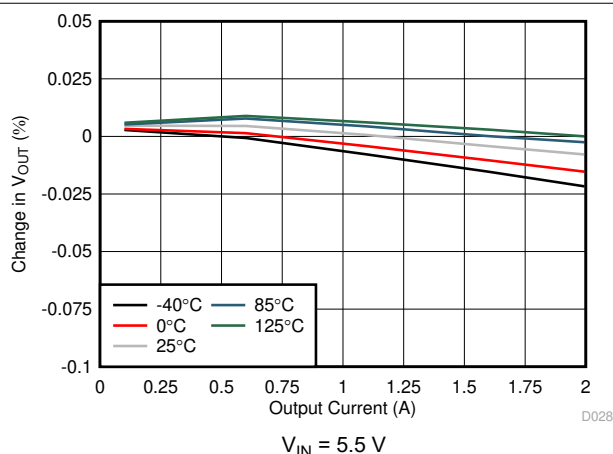
FIG 7-28. Load Regulation (5-V Output)
