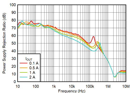
FIG 7-43. PSRR vs Frequency and I_{OUT}
