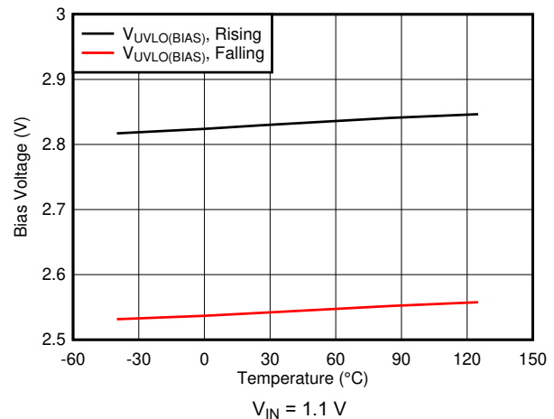
FIG 7-38. V_{BIAS} UVLO vs Temperature
