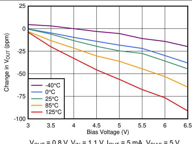
FIG 7-30. Line Regulation With BIAS
