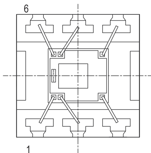
図 11-1. Package Orientation Visual Reference of Pin 1 (Top View)
