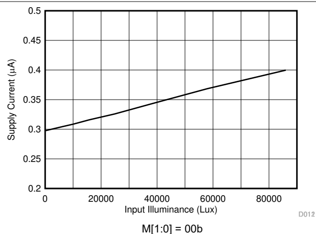
5-17. Shutdown Current vs Input Illuminance
