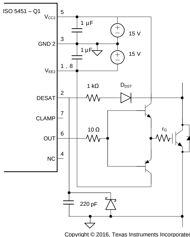
Figure 51. Current Buffer for Increased Drive Current
