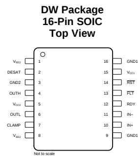
Pin Functions
