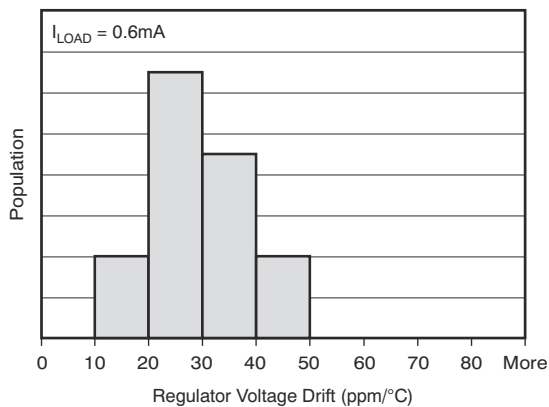
図 5-25. Regulator Voltage Drift Distribution
