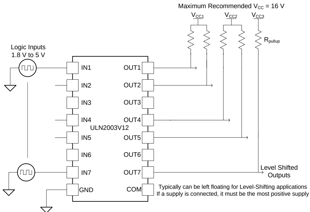
Figure 6. ULN2003V12 as Inverting Logic Level Shifter
