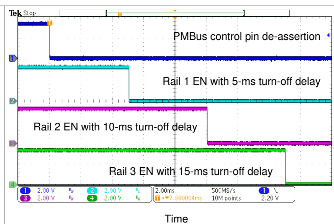
Figure 42. Shut-Down Waveforms
