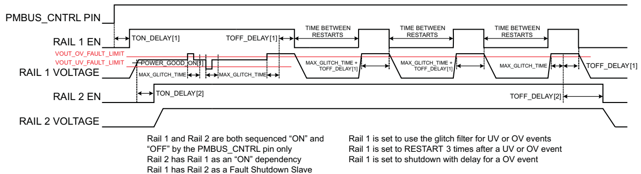
FIG 16. Sequencing and Fault-Response Timing
