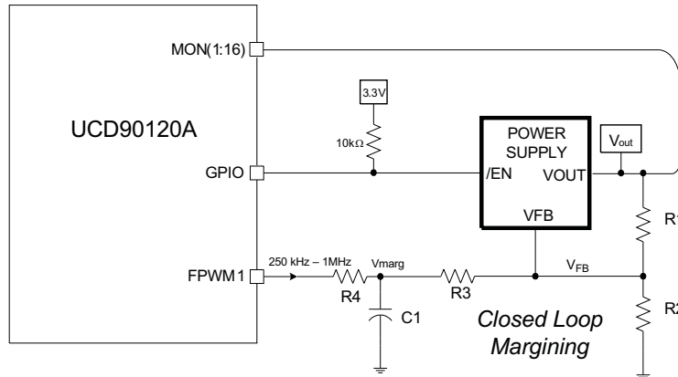
图 24. Closed-Loop Margining
