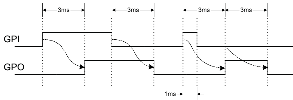
FIG 21. GPO Behavior When Ignoring Inputs During Delay
