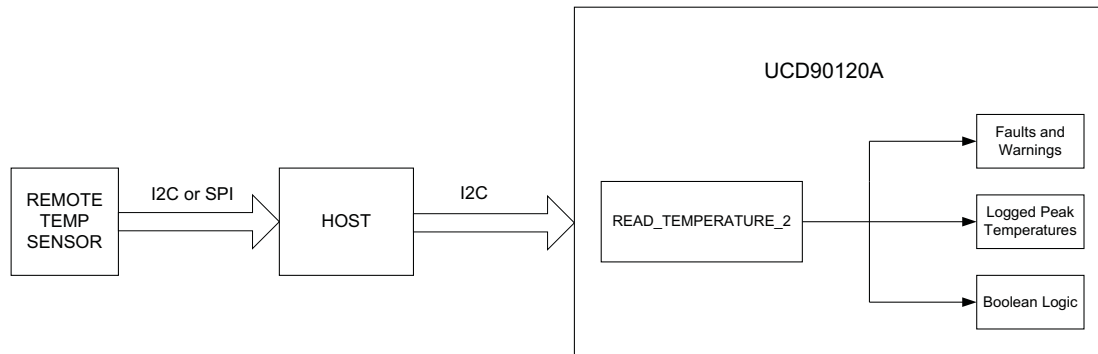
FIG 15. Temperature Provided by Host
