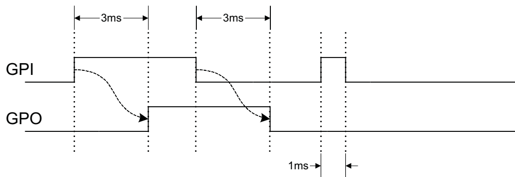
FIG 20. GPO Behavior When Not Ignoring Inputs During Delay
