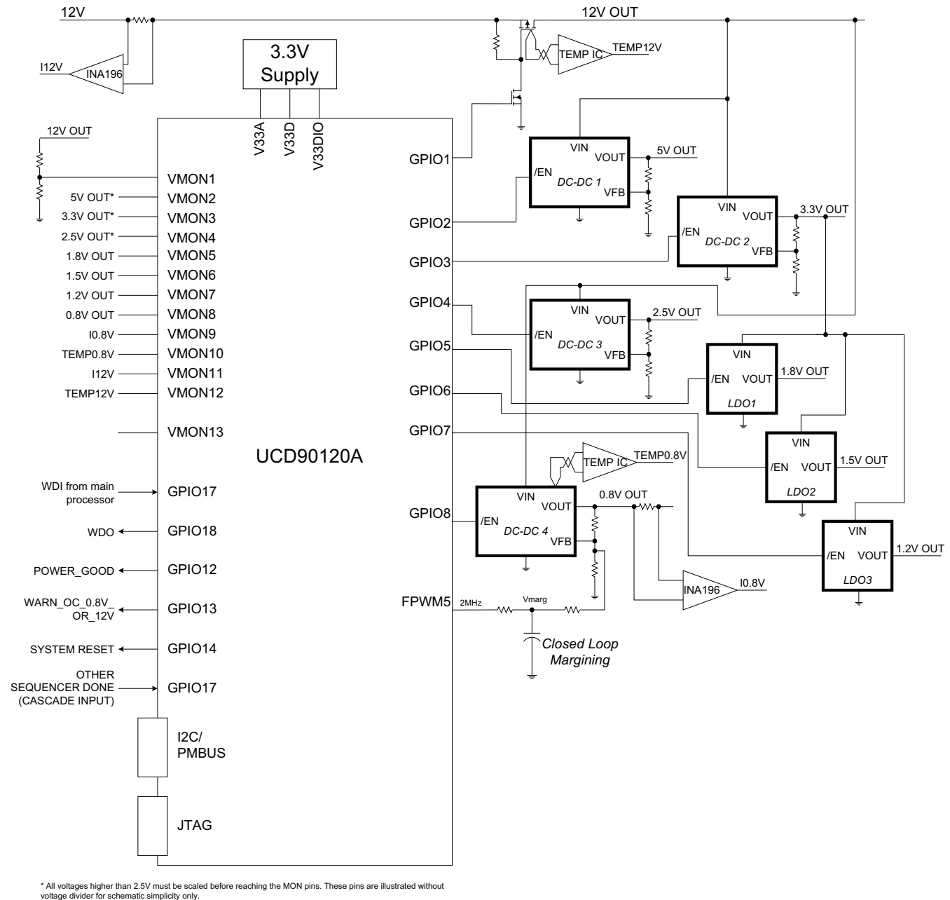
32. Typical Application Schematic
