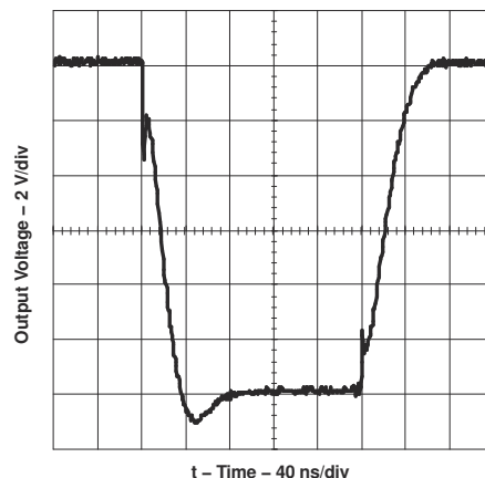
FIG 10-2. Output Rise and Fall Time ( V_{DD} = 12 V, C_{LOAD} = 10 nF)
