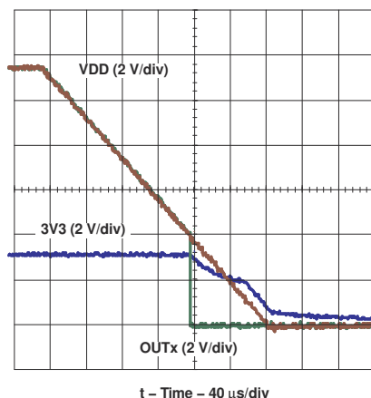
8-16. Shut Down Behavior at V_{DD} = 12 V (Input Tied to 3V3)
