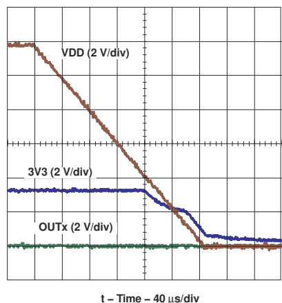
8-18. Shut Down Behavior at V_{DD} = 12 V (Input Shortened to GND)
