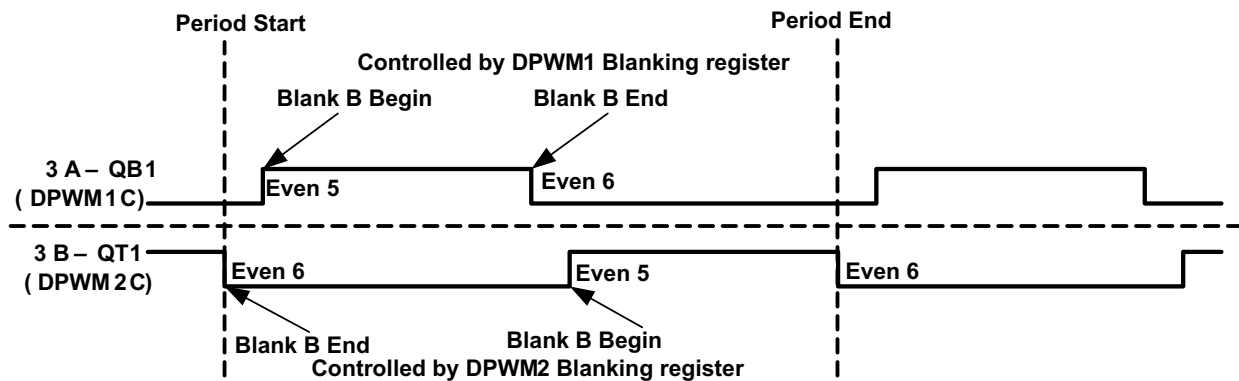
FIG 10-5. Blank B Timing Information
