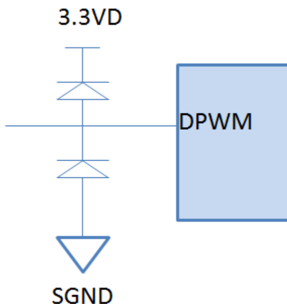
FIG 12-4. Clamping Diodes for DPWM
