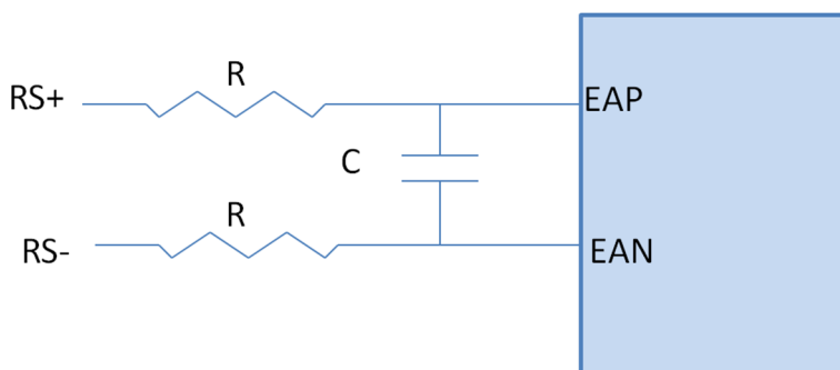
FIG 12-5. Local Filter on EAPx and EANx Pins
