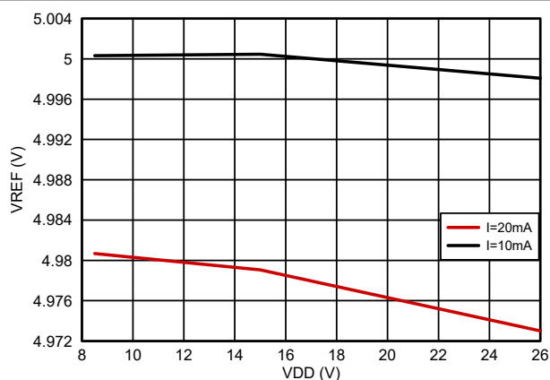
Figure 5-20. Vref Voltage vs VDD
