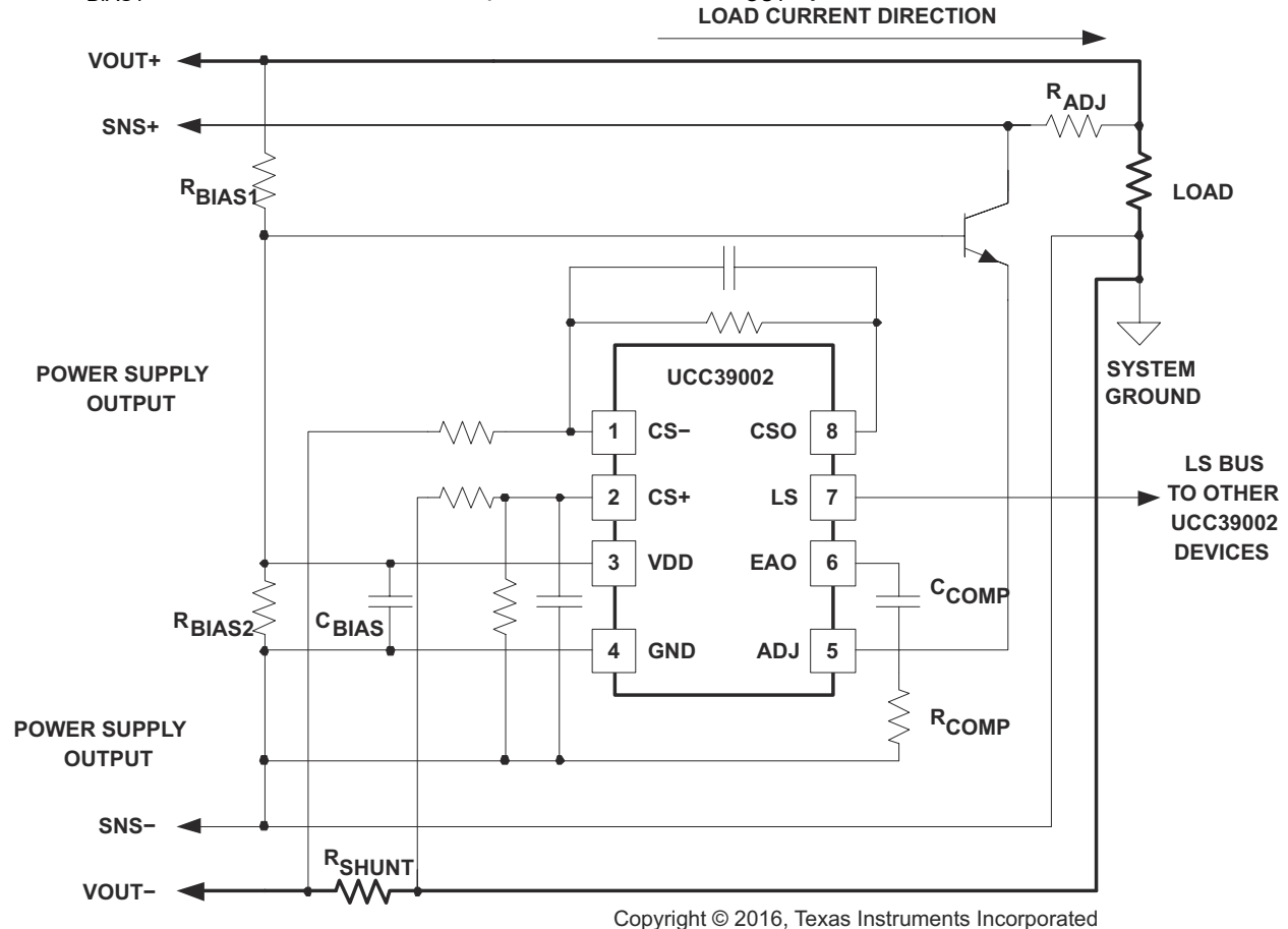
7-2. High-Voltage Application with Low-side Current-Sensing
