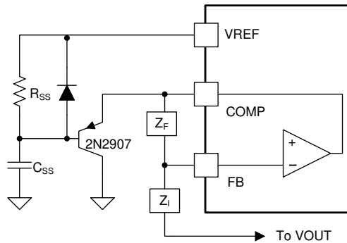
8-6. Soft-Start Implementation
