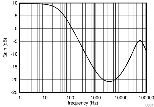
Figure 9-4. Converter Open-Loop Bode Plot - Gain
