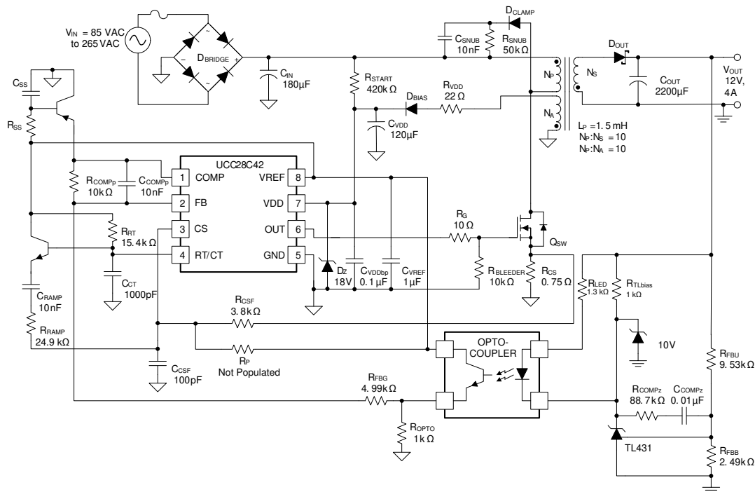
9-3. Typical Application Design Schematic
