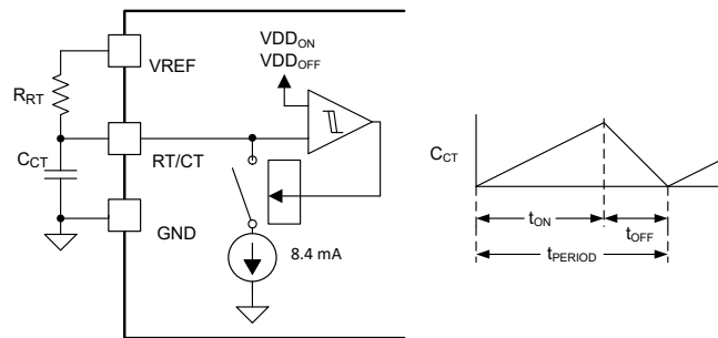
FIG 8-4. Oscillator Circuit
