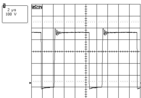
9-8. Primary Side MOSFET Drain to Source Voltage at 240-V AC Input (100 V/div)
