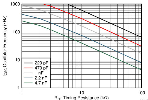
7-1. Oscillator Frequency vs Timing Resistance and Capacitance
