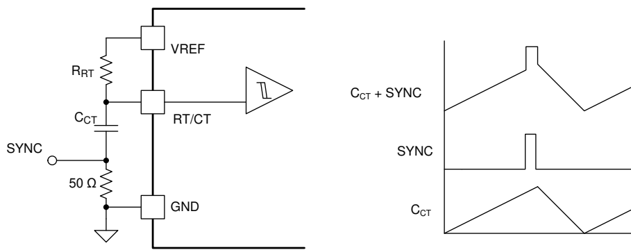
FIG 8-5. Oscillator Synchronization Circuit
