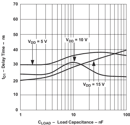
図 7-13. t_{D1} Delay Time vs Load Capacitance
