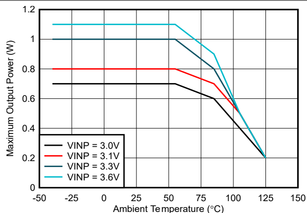
Figure 6-2. Maximum Output Power vs Ambient Temperature : VCC = 5.0V , C OUT2 = 22µF
