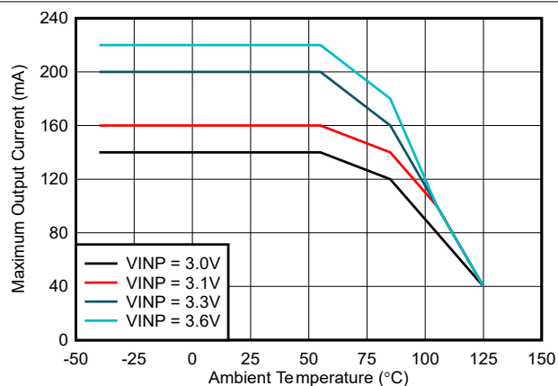
Figure 6-6. Maximum Output Current vs Ambient Temperature : VCC = 5.0V , C OUT2 = 22µF
