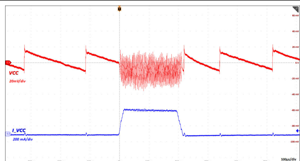
図 6-27. Load Transient: VINP = 5.0V, VCC = 5.0V , C OUT2 = 22µF , I VCC = 0mA - 300mA - 0mA
