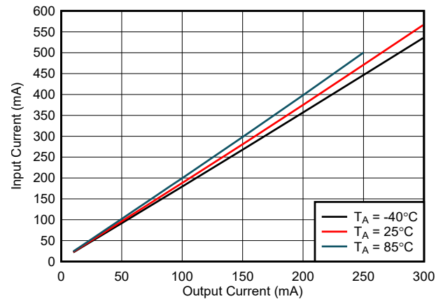
図 6-16. Input Current ( I_{VINP} ) vs Load Current ( I_{VCC} ): V_{CC} = 5.0V , V_{INP} = 5.0V , C_{OUT2} = 22\mu F
