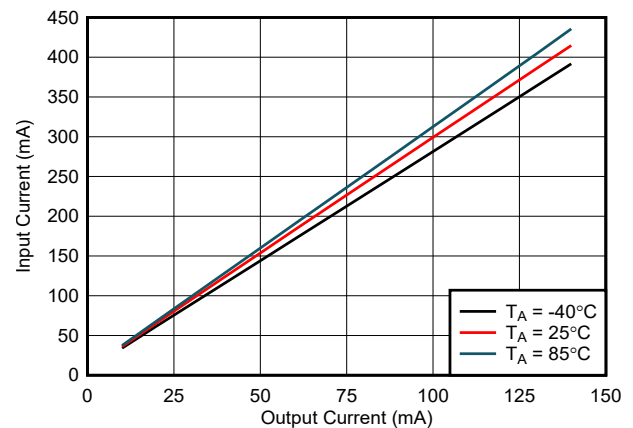
図 6-18. Input Current ( I_{VINP} ) vs Load Current ( I_{VCC} ): V_{CC} = 5.0V , V_{INP} = 3.3V , C_{OUT2} = 22\mu F
