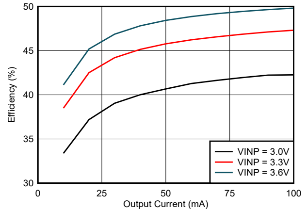
図 6-14. Efficiency vs Load Current ( I_{VCC} ): V_{CC} = 5.5V , T_A = 25^\circ C , C_{OUT2} = 22\mu F
