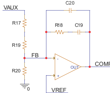
FIG 9-4. Type-II Compensation with an Error Amplifier
