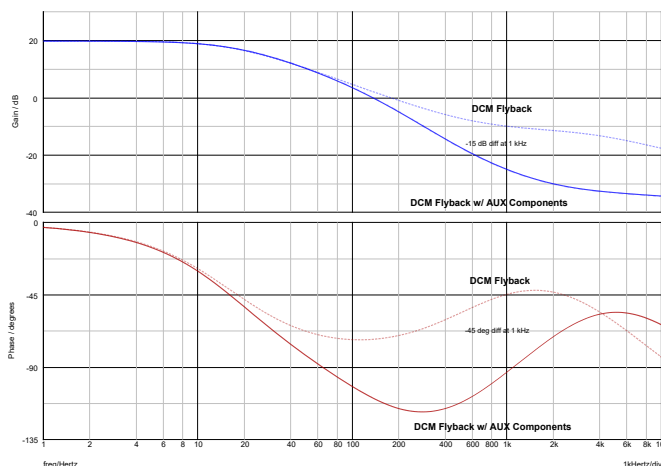
FIG 9-3. Comparison of DCM Flyback Plant with and without AUX Components
