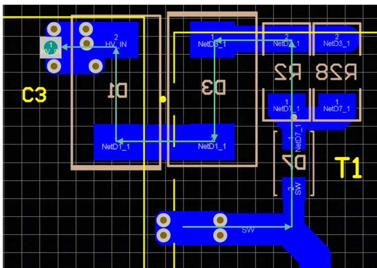
9-27. High-Voltage Clamp Loop Routing
