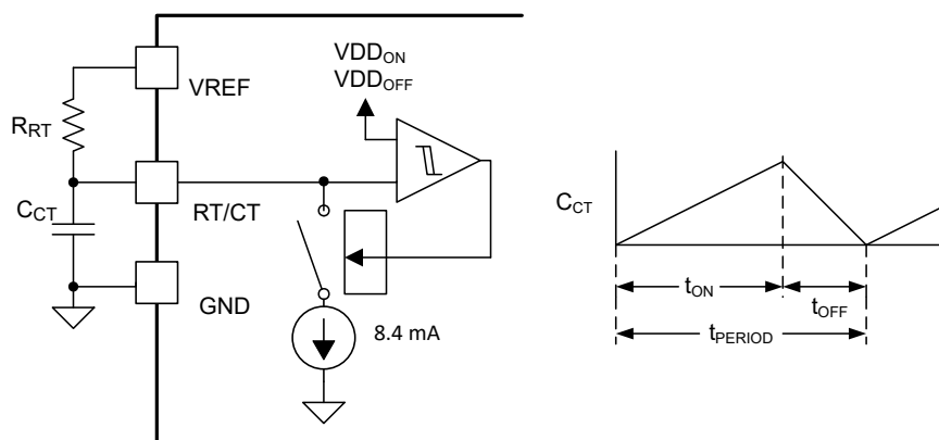
FIG 8-4. Oscillator Circuit
