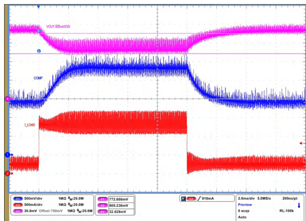
9-18. PWM Switching at 50 V IN , 20 W
