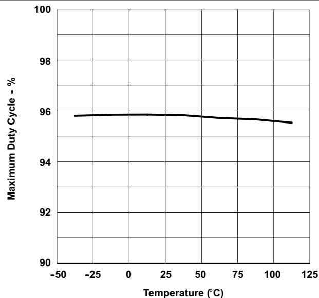
Figure 7-19. Maximum Duty Cycle vs Temperature
