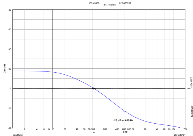
FIG 9-5. Measuring the plant gain at the desired crossover frequency: -23 dB at 625 Hz
