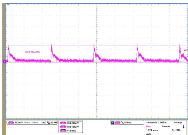
9-14. V_{OUT} Overshoot at 50 V_{IN} , 20W
