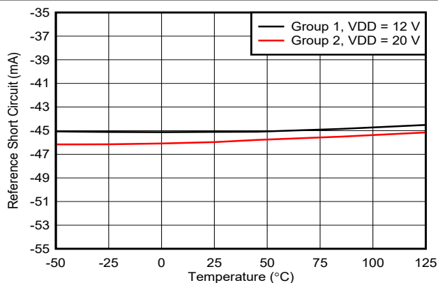
7-7. Reference Short-Circuit Current vs Temperature
