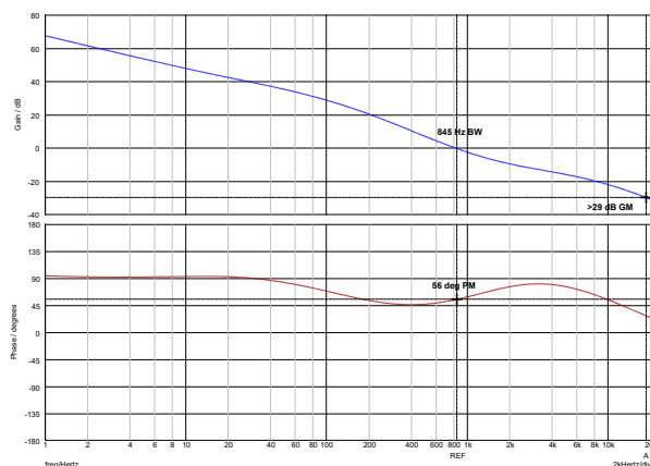
Figure 9-7. 40 V IN , Maximum Load (1.33 A)
