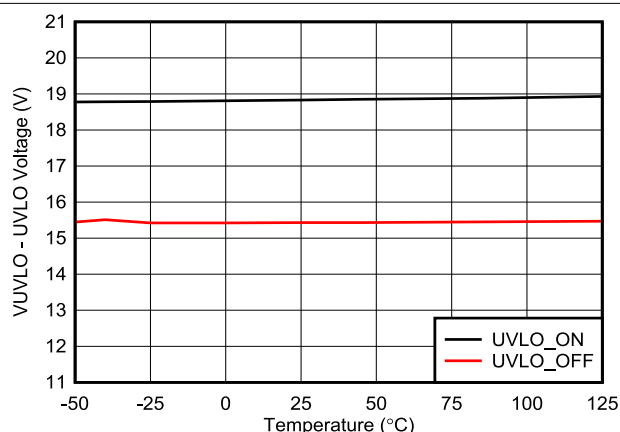
7-10. Undervoltage Lockout vs Temperature
