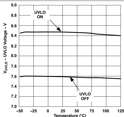
7-10. Undervoltage Lockout vs Temperature
