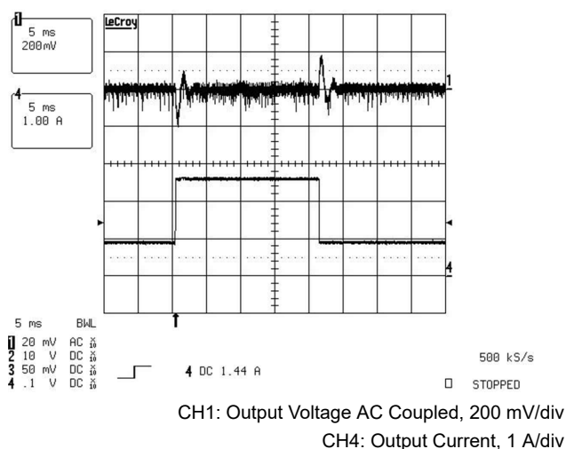
9-9. Output Voltage During 0.9-A to 2.7-A Load Transient
