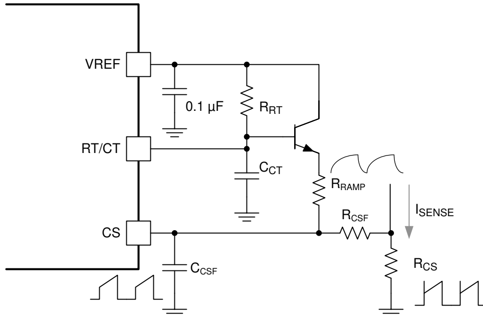
Figure 8-8. Slope Compensation Circuit
