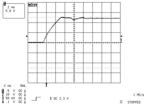
9-11. Output Voltage Behavior at Full Load Start-up (5 V/div)
