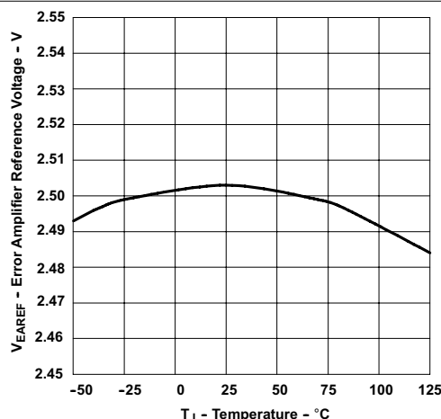
7-6. Error Amplifier Reference Voltage vs Temperature
