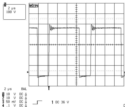
9-7. Primary Side MOSFET Drain to Source Voltage at 240-V AC Input (100 V/div)
