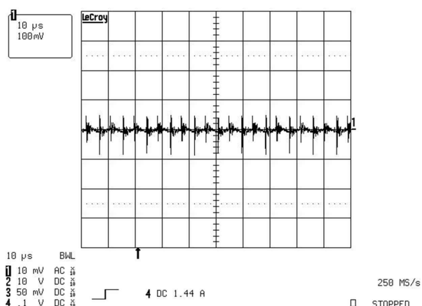
9-10. Output Voltage Ripple at Full Load (100 mV/div)
