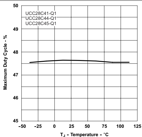
7-17. Maximum Duty Cycle vs Temperature
