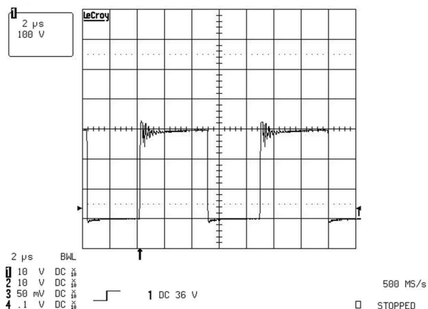
9-8. Primary Side MOSFET Drain to Source Voltage at 120-V AC Input (100 V/div)
