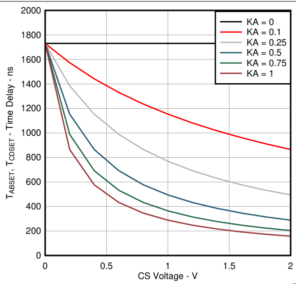
Figure 6-3. Delay Time set T_{ABSET} and T_{CDSET} (Over CS Voltage Variation and Selected K_A for R_{AB} and R_{CD} Equal 90 kΩ)
