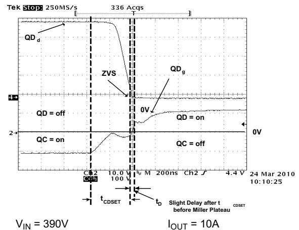
7-14. Full-Bridge Gate Drives and Switch Nodes (QD g QD d )
