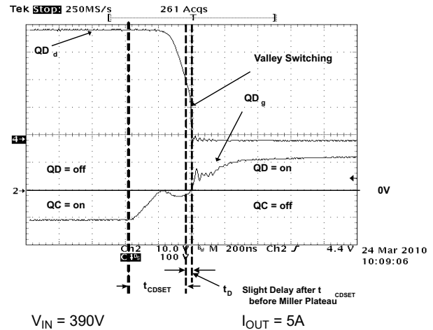
7-12. Full-Bridge Gate Drives and Primary Switch Nodes (QD g QD d )
