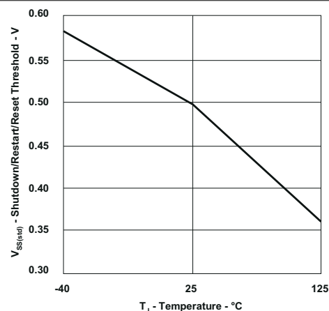
5-16. Shutdown, Restart, and Reset Threshold vs Temperature
