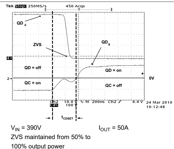
Figure 7-18. Full-Bridge Gate Drives and Switch Nodes (QD g QD d )
