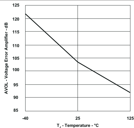
5-14. Voltage Error Amplifier (Open-Loop Gain) vs Temperature
