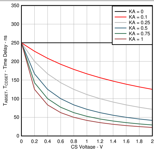
Figure 6-2. Delay Time Set T_{ABSET} and T_{CDSET} (Over CS Voltage Variation and selected K_A for R_{AB} and R_{CD} Equal 13kΩ)
