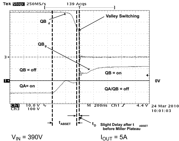
7-11. Full-Bridge Gate Drives and Primary Switch Nodes (QB d and QD d )
