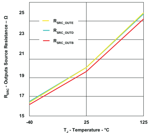
図 5-24. Outputs Source Resistance vs Temperature
