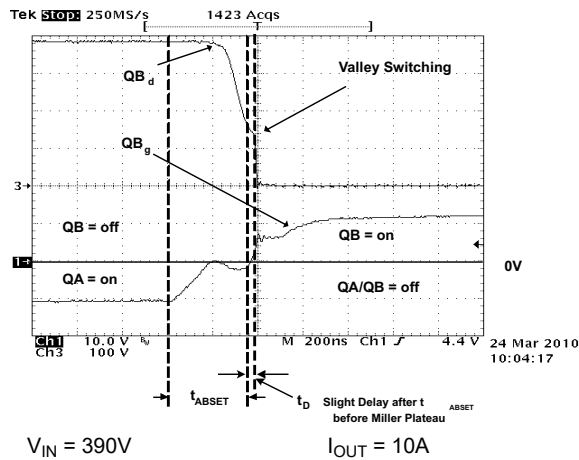
7-13. Full-Bridge Gate Drives and Switch Nodes (QB g QB d )
