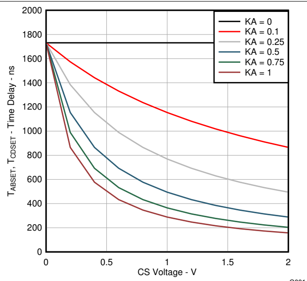
Figure 6-3. Delay Time set T_{ABSET} and T_{CDSET} (Over CS Voltage Variation and Selected K_A for R_{AB} and R_{CD} Equal 90 kΩ)
