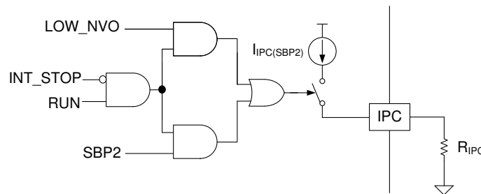
FIG 7-9. Control Circuit Diagram to the IPC-Pin Current Source
