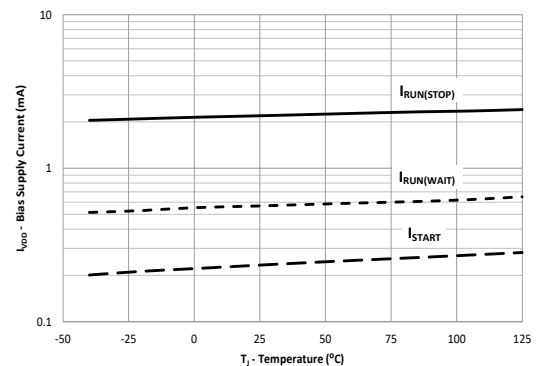
6-2. VDD Bias-Supply Current vs. Temperature
