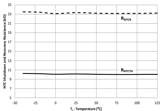
6-11. FLT OTP Thresholds vs. Junction Temperature
