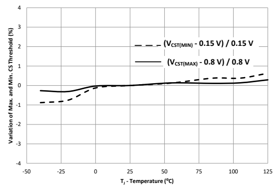
6-4. Percentage Variation of Maximum and Minimum CS Thresholds vs. Temperature
