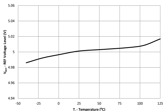
6-9. REF Voltage vs. Temperature
