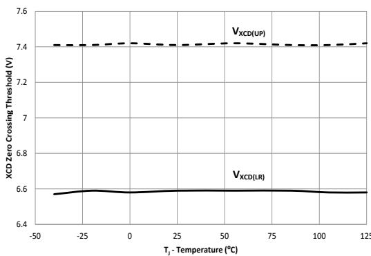
6-12. XCD Thresholds vs. Junction Temperature
