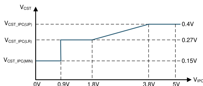
FIG 7-10. IPC Transfer Function to Program the SBP2 Peak Current Threshold
