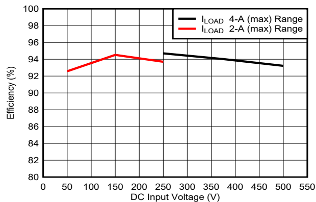
8-6. Full-Load Efficiency vs. DC Input Voltage
