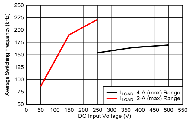
8-7. Average Switching Frequency at Full-Load vs. DC Input Voltage
