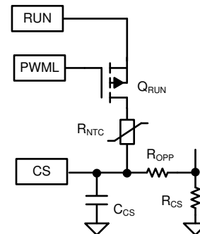
FIG 7-42. Two Connections to Implement OTP on the CS Pin
