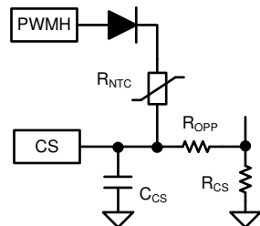
FIG 7-42. Two Connections to Implement OTP on the CS Pin
