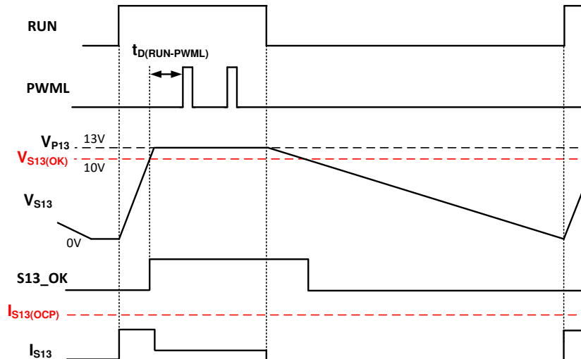
FIG 7-7. Power Management Function for a GaN Power IC and PFC Controller
