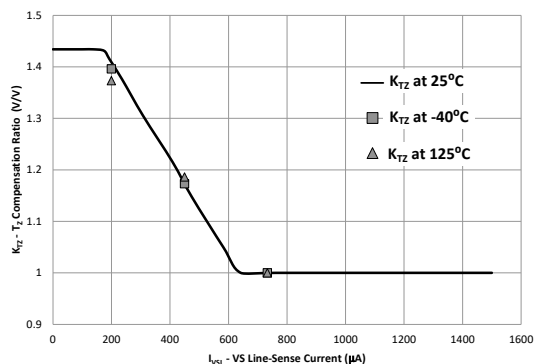
6-7. t_Z Compensation Ratio ( K_{TZ} ) vs. VS Line-Sense Currents
