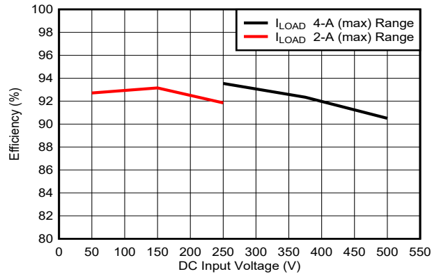
8-4. 4pt-Average Efficiency vs. DC Input Voltage
