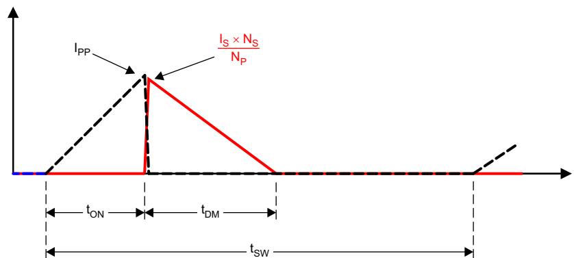
Figure 7-6. Transformer-Current Relationship
