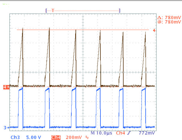
8-5. EMI Dithering
