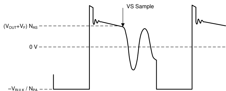
✎ 7-3. Auxiliary-Winding Voltage
