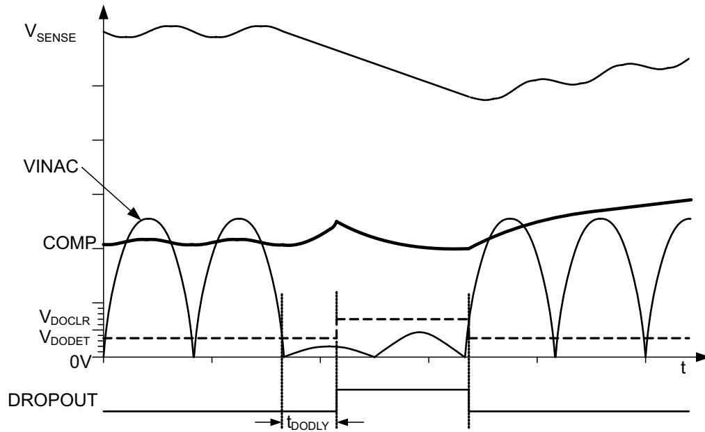
⊠ 29. AC-Line Dropout Timing With Illustrative System Behavior
