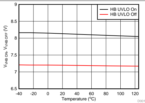
FIG 14. VHB-VHS UVLO Thresholds vs Temperature
