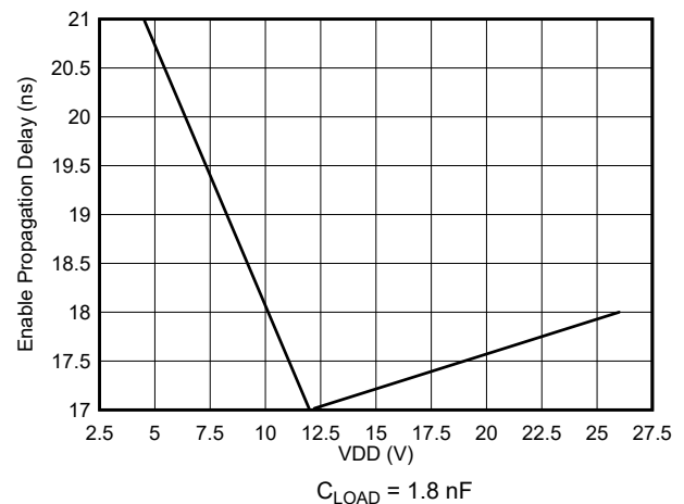
図 5-20. Enable to Output Rising Propagation Delay
