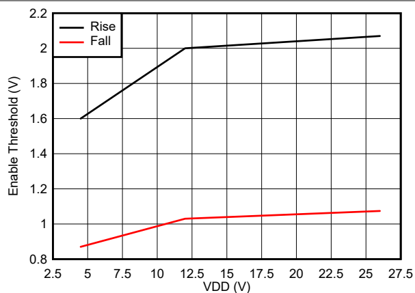
Figure 5-10. Enable Threshold
