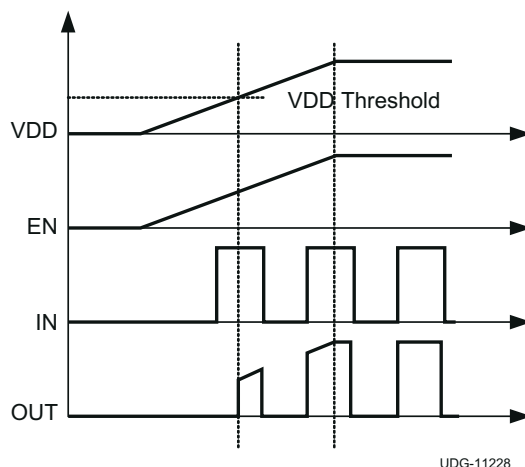
図 7-2. Power-Up Sequence
