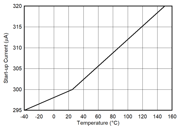
図 5-3. Start-Up and Quiescent Current
