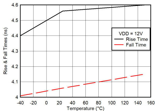
6-8. Output Rise and Fall Time vs Temperature
