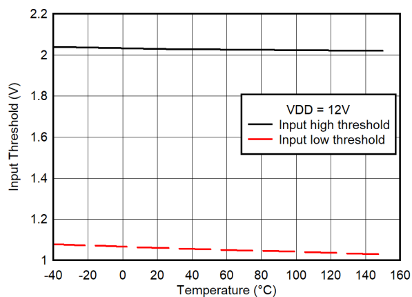
6-15. Input Threshold vs Temperature
