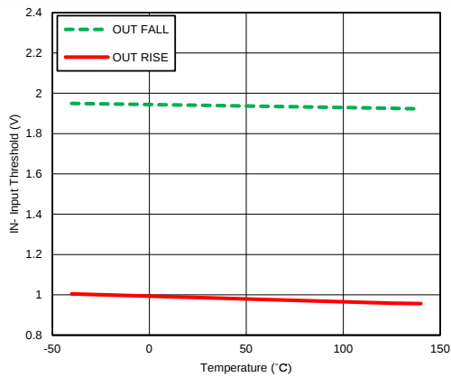
FIG 18. In- Input Threshold vs. Temperature
