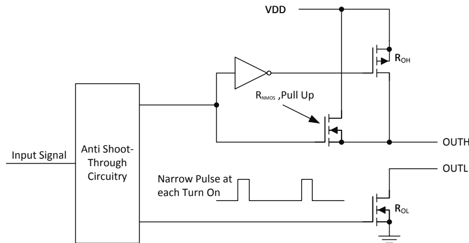
FIG 39. UCC27531 Gate Driver Output Stage
