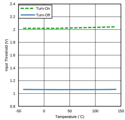
FIG 17. Input Threshold vs. Temperature
