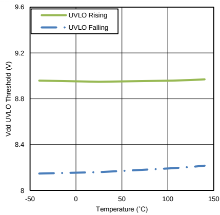
FIG 16. UVLO Threshold Voltage vs. Temperature
