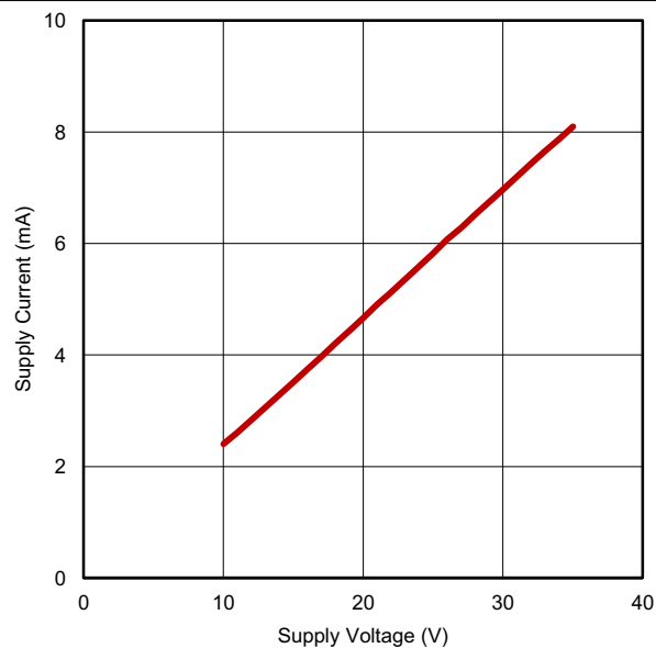
図 5-17. Operating Supply Current vs Supply Voltage (output switching)
