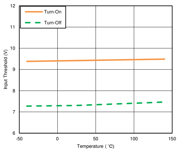
Figure 5-9. Input Threshold vs Temperature
