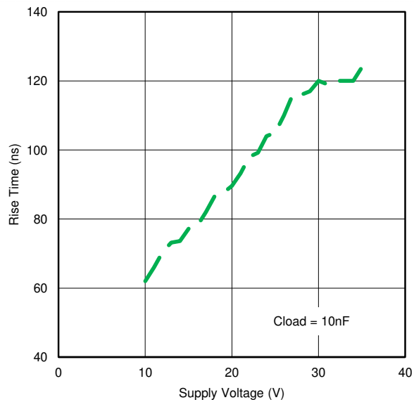
5-18. Rise Time vs Supply Voltage
