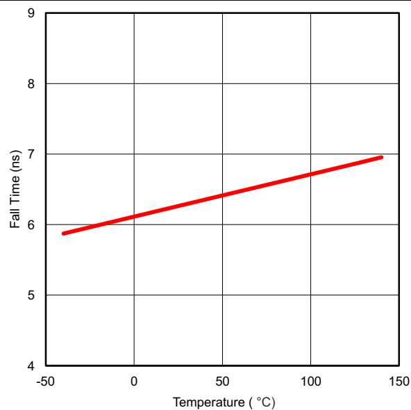
図 5-16. Fall Time vs Temperature
