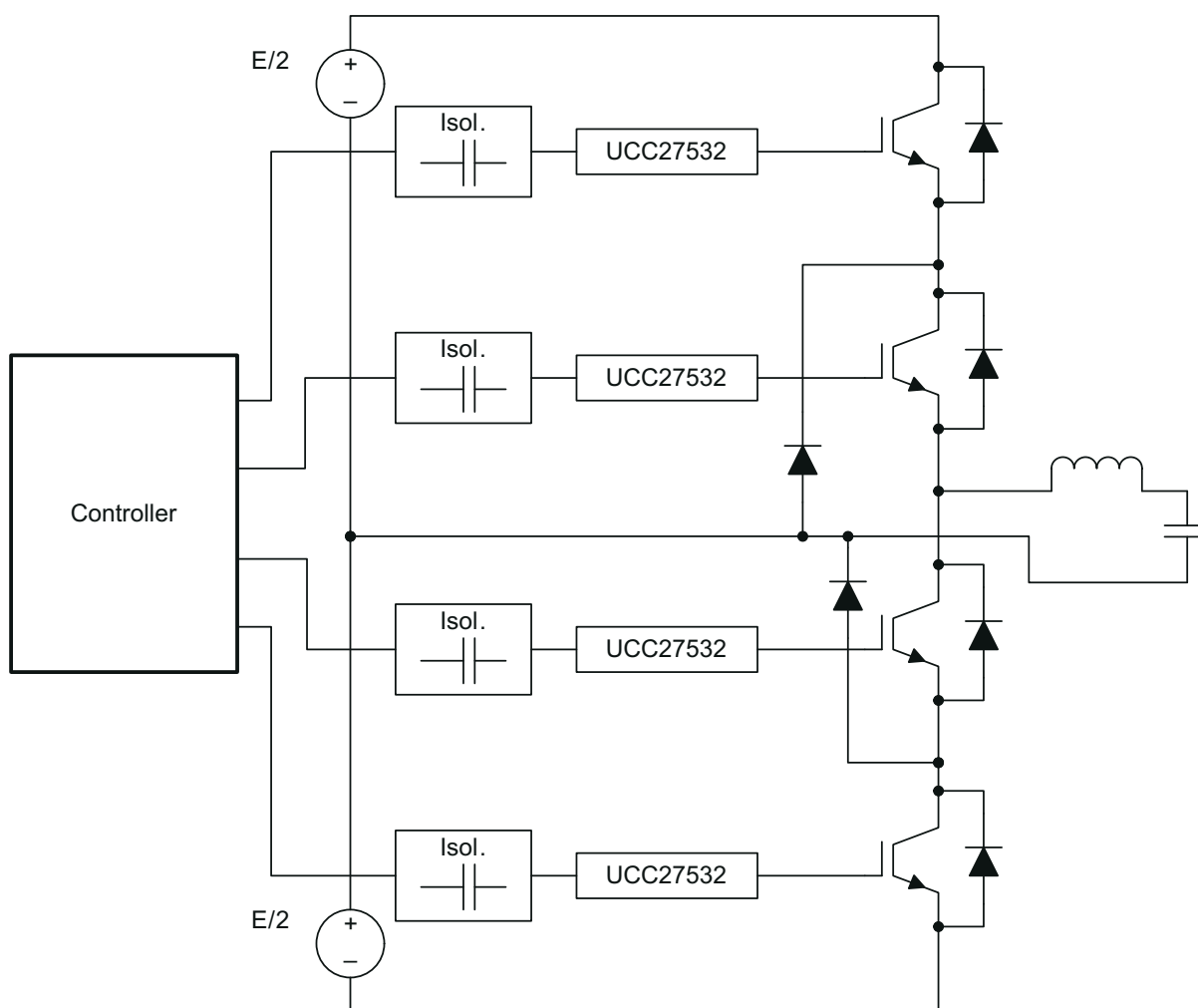
図 7-3. Using UCC27532 Drivers in an Inverter
