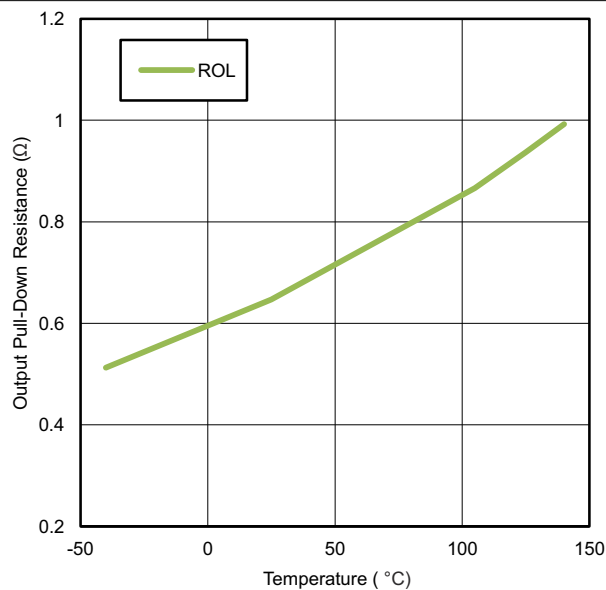
図 5-12. Output Pull-Down Resistance vs Temperature
