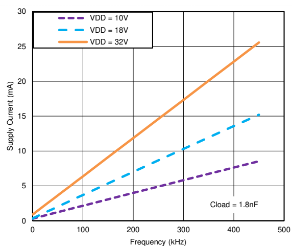
図 5-5. Operating Supply Current vs Frequency
