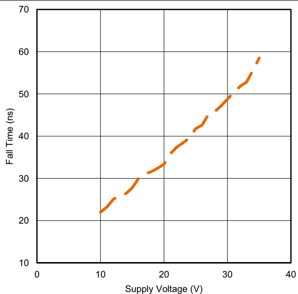
5-19. Fall Time vs Supply Voltage
