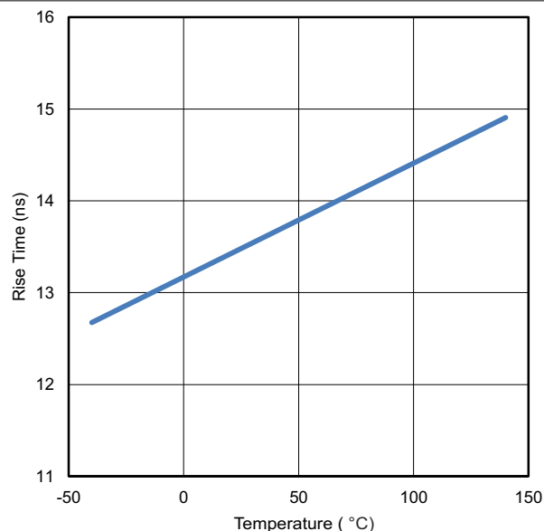
図 5-15. Rise Time vs Temperature
