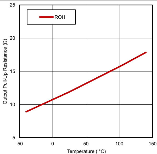
図 5-11. Output Pull-Up Resistance vs Temperature
