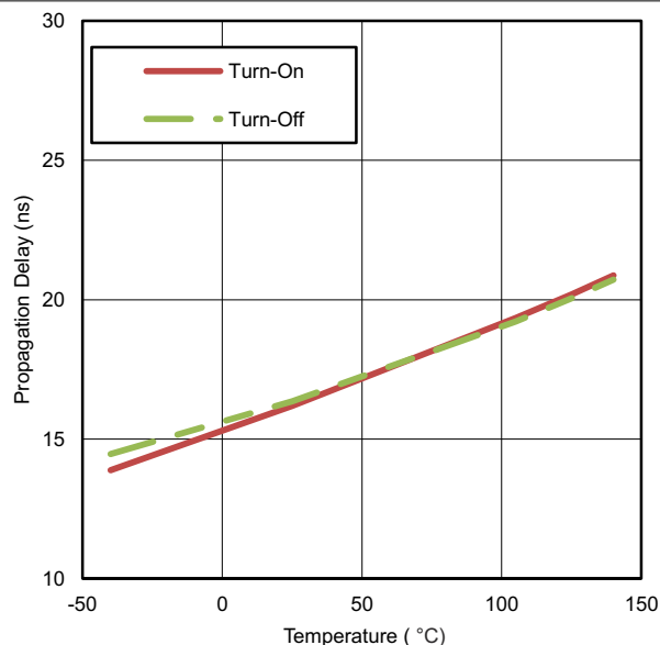
図 5-14. Input-to-Output Propagation Delay vs Temperature
