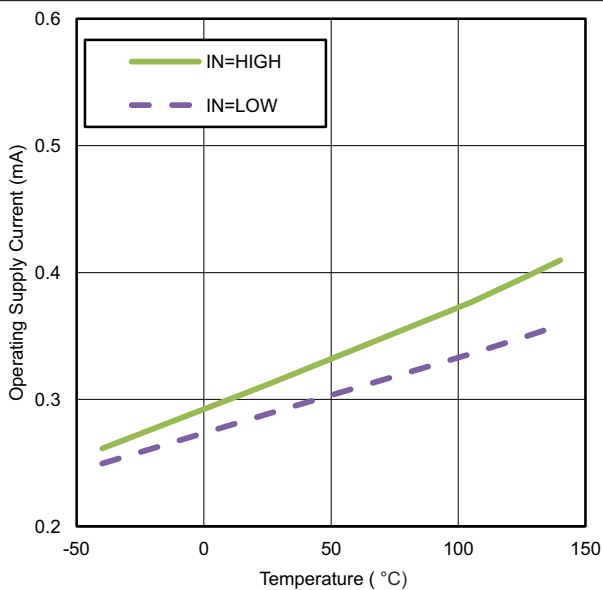
図 5-13. Operating Supply Current vs Temperature (output in DC on/off condition)
