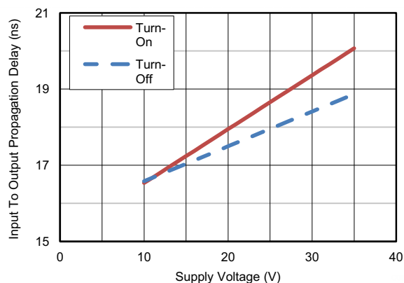
図 5-4. Propagation Delay vs Supply Voltage
