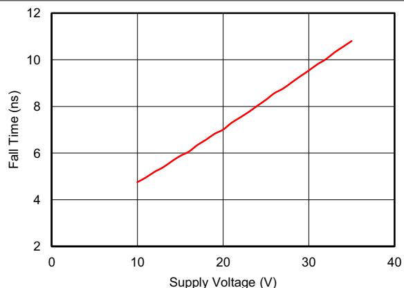
図 5-3. Fall Time vs Supply Voltage
