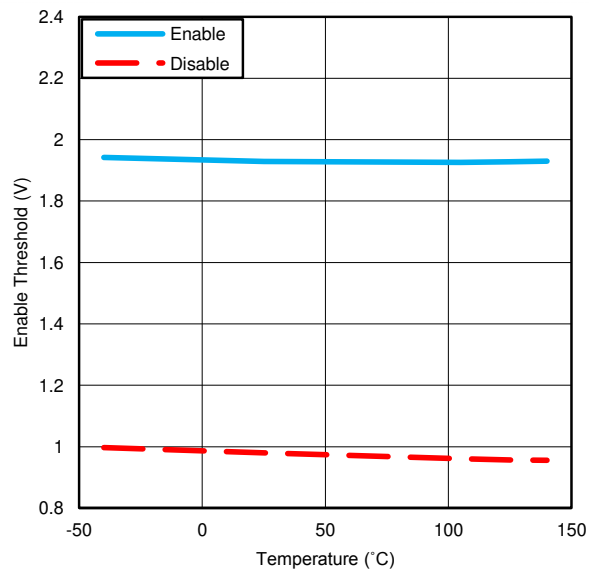
図 5-10. Enable Threshold vs Temperature
