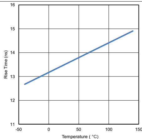
Figure 17. Rise Time vs Temperature
