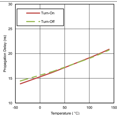
Figure 15. Input-to-Output Propagation Delay vs Temperature
