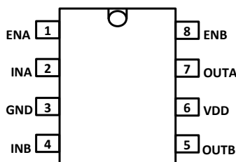
図 5-1. D Package 8-Pin SOIC Top View
