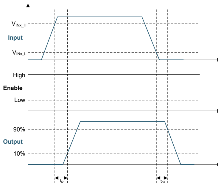
ⓧ 6-2. Input-Output Operation
