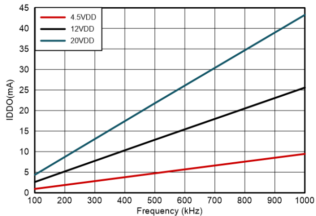
FIG 6-4. Operating Supply Current (both outputs switching)
