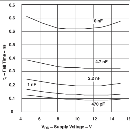
図 6-15. Fall Time vs Supply Voltage
