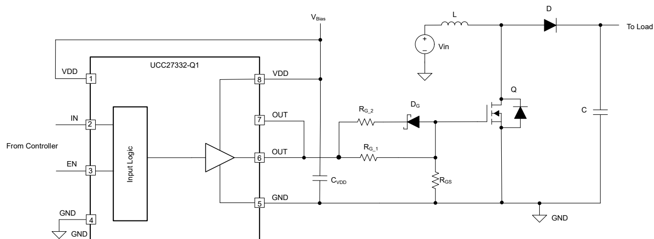
8-1. Driving a MOSFET in a Boost Converter
