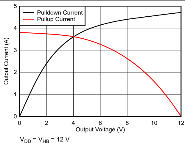
Figure 5-17. Output Current vs Output Voltage
