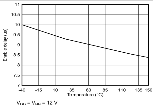
Figure 5-15. Enable delay vs Temperature
