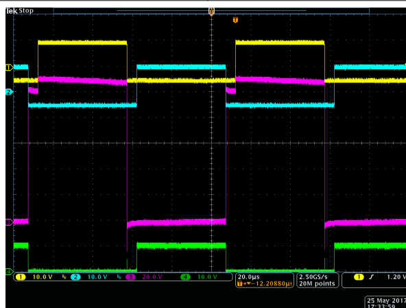
8-8. Propagation Delay and Delay Matching
