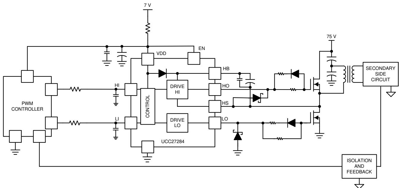
图 8-1. Typical Application
