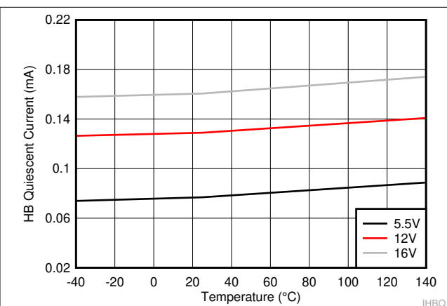
6-2. HB Quiescent Current
