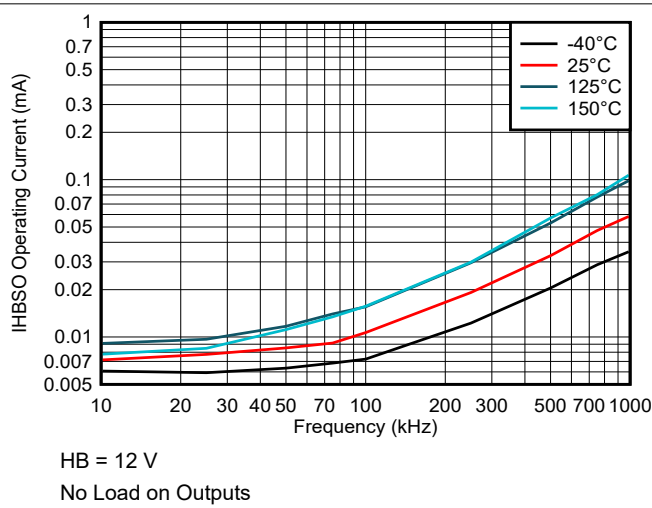
Figure 5-5. HB to VSS Operating Current vs Frequency
