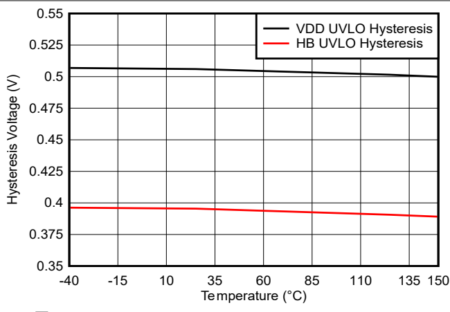
FIG 5-13. Undervoltage Lockout Threshold Hysteresis vs Temperature
