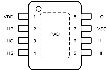
図 4-2. DDA Package 8-Pin SO PowerPAD Top View
