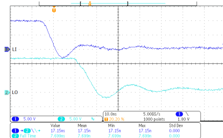
図 7-3. LO Fall Time and LI to LO Turn-off Propagation Delay
