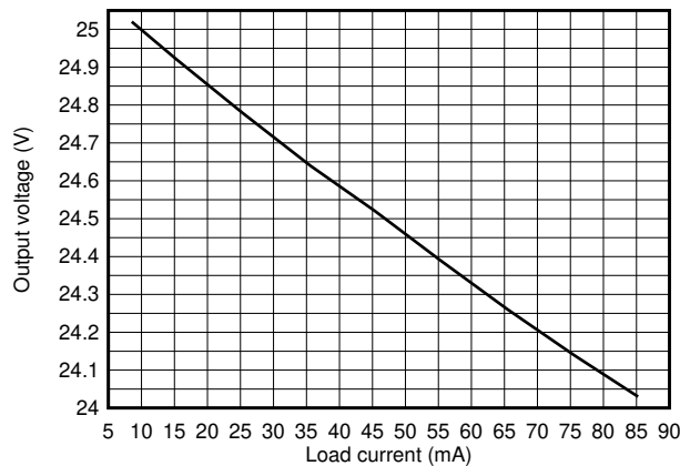
Figure 9-10. LLC output voltage load regulation
