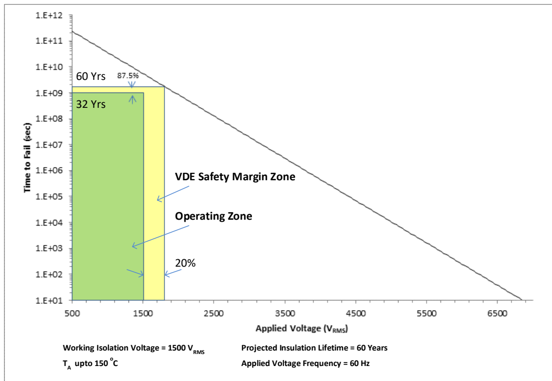
6-3. Reinforced Isolation Capacitor Life Time Projection
