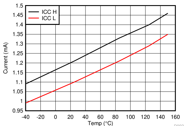
Figure 6-5. Supply currents versus Temperature
