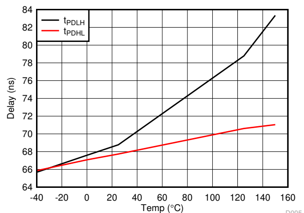
Figure 6-8. Propagation delay versus Temperature
