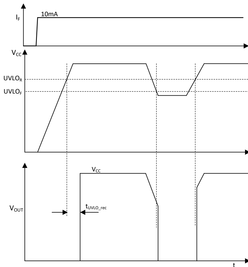
FIG 8-5. UVLO functionality
