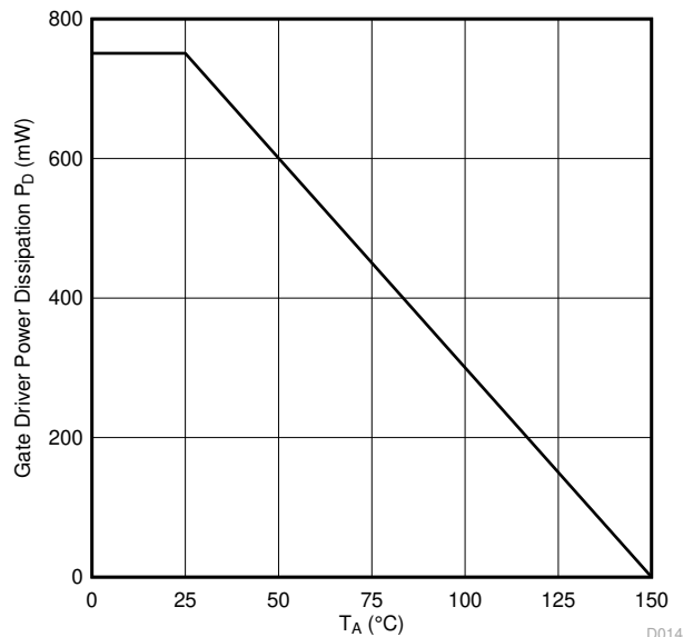
6-2. Thermal Derating Curve for Limiting Power per VDE
