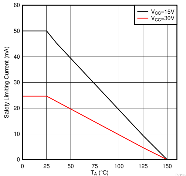
6-1. Thermal Derating Curve for Limiting Current per VDE
