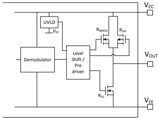
✎ 8-4. Output Stage
