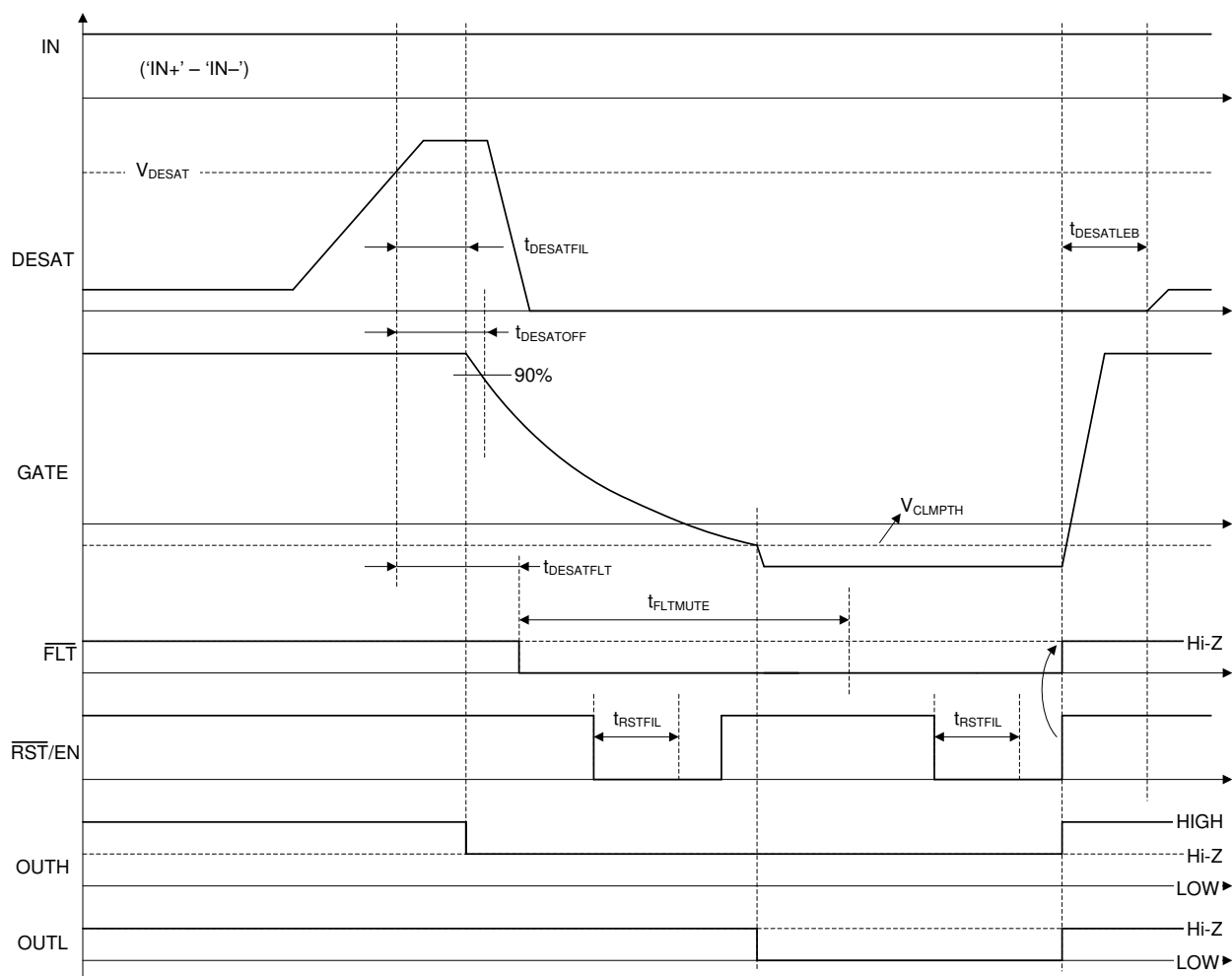
図 6-11. DESAT Protection with Soft Turn-OFF While Power Device is ON
