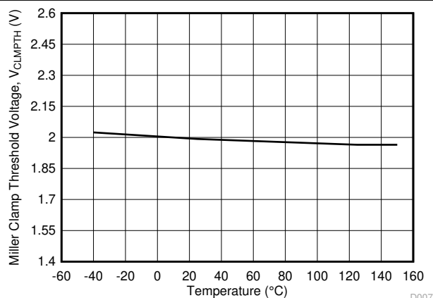
图 5-20. V_{CLMPH} Miller Clamp Threshold Voltage vs Temperature
