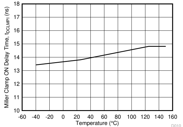
FIG 5-22. t_{DCLMPI} Miller Clamp ON Delay Time vs Temperature
