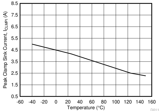
FIG 5-21. I_{CLMPI} Miller Clamp Sink Current vs Temperature
