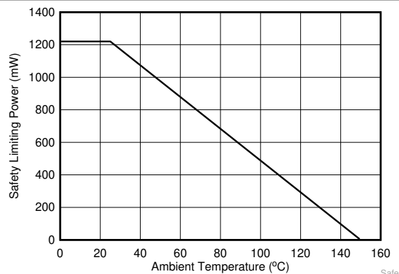
図 5-2. Thermal Derating Curve for Limiting Power per VDE
