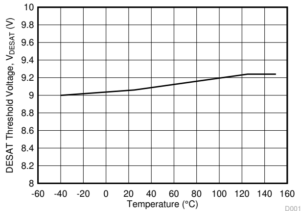
FIG 5-23. V_{DESAT} DESAT Threshold Voltage vs Temperature
