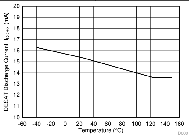
図 5-29. I_{\text{DCHG}} DESAT Discharge Current vs Temperature
