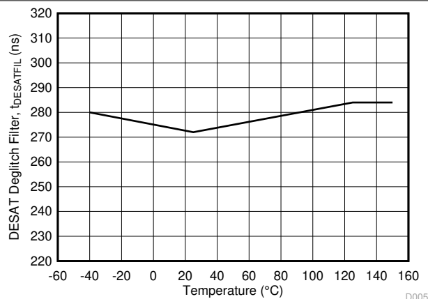
図 5-27. t_{\text{DESATFIL}} DESAT Deglitch Filter vs Temperature
