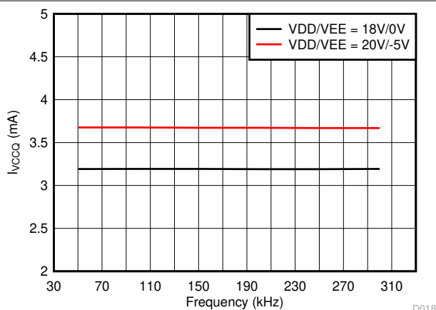
図 5-7. I_{VCCQ} Supply Current vs Input Frequency
