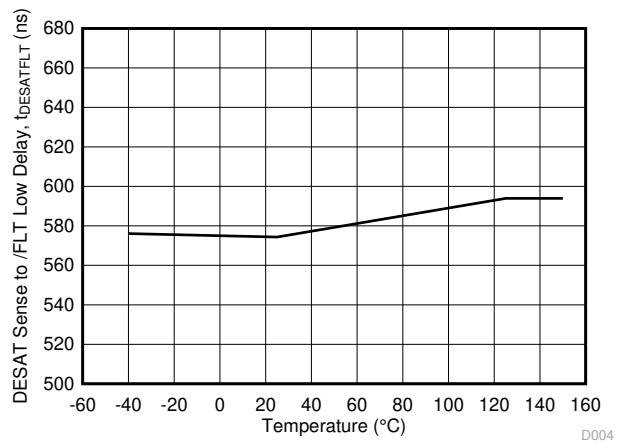
FIG 5-26. t_{DESATFLT} DESAT Sense to /FLT Low Delay Time vs Temperature
