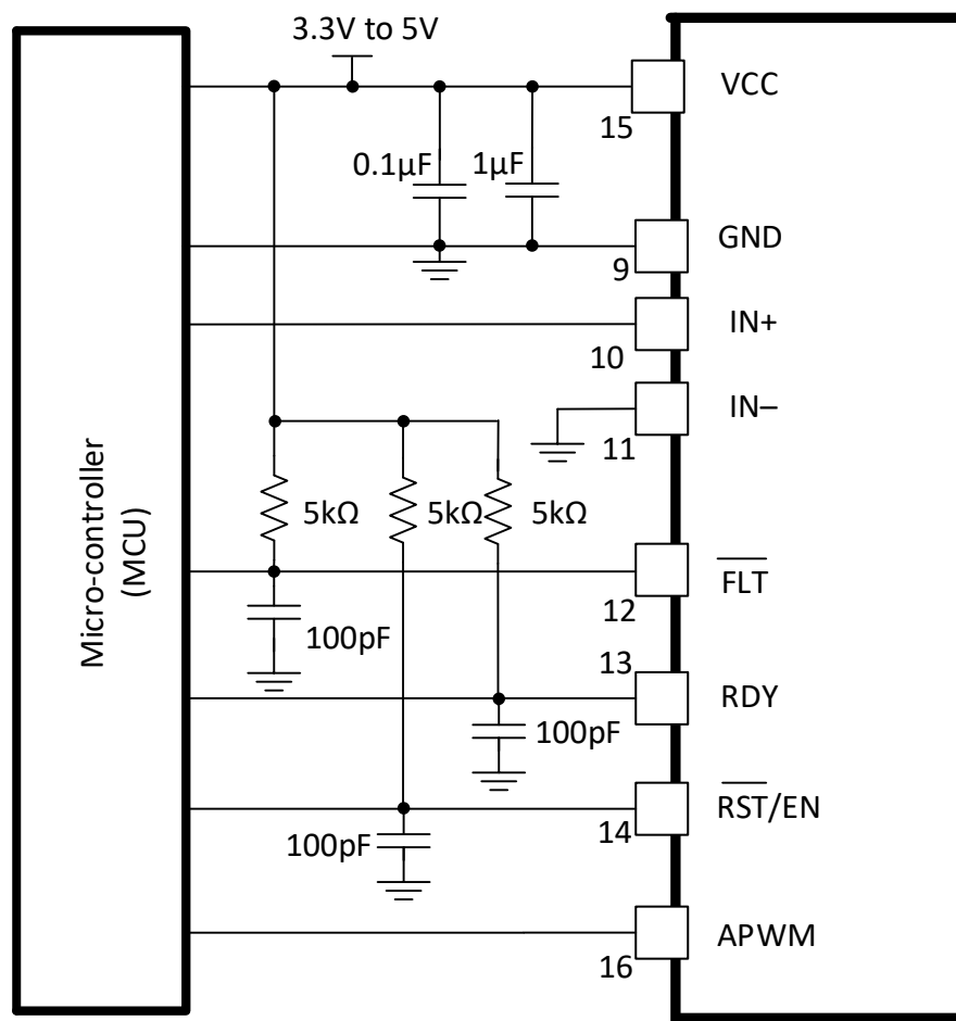
8-3. FLT, RDY and RST/EN Pins Circuitry
