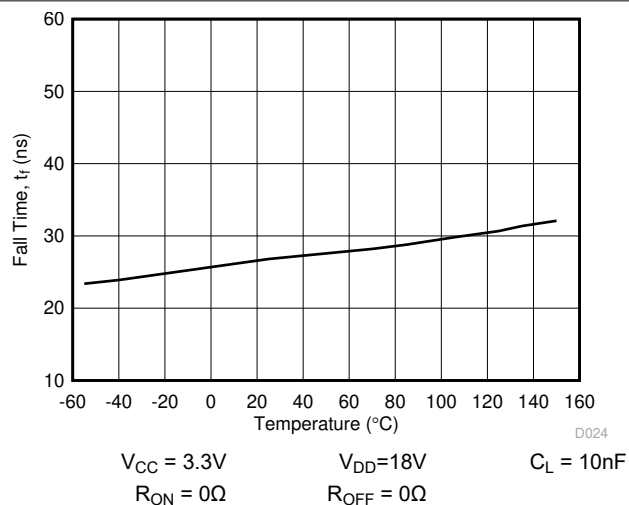
图 5-16. t_f Fall Time vs Temperature
