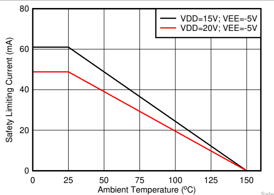
図 5-1. Thermal Derating Curve for Limiting Current per VDE
