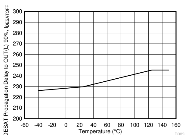
FIG 5-25. t_{DESATOFF} DESAT Propagation Delay to OUT(L) 90% vs Temperature
