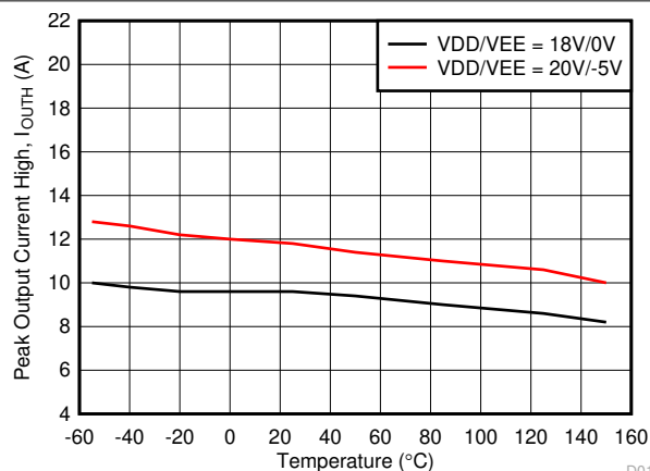
図 5-3. Output High Drive Current vs Temperature
