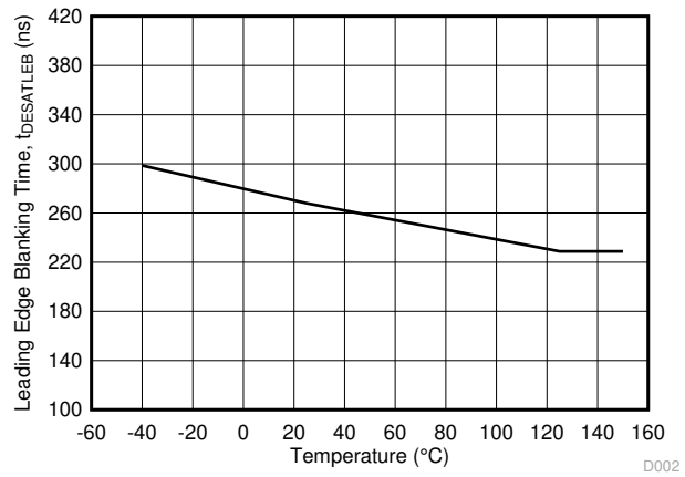
FIG 5-24. t_{DESATLEB} DESAT Leading Edge Blanking Time vs Temperature
