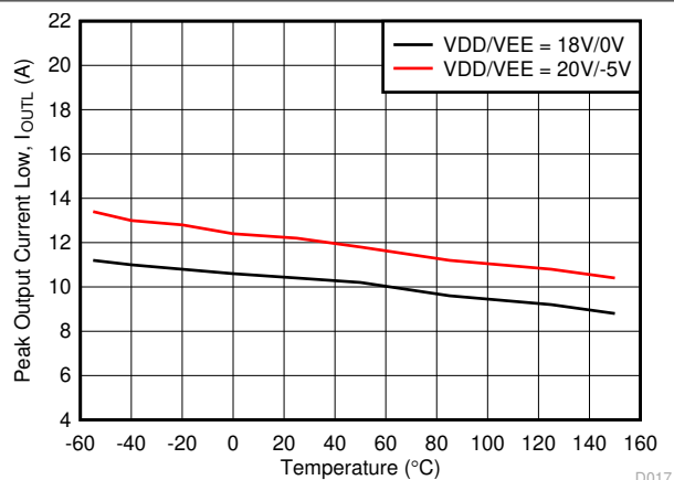
図 5-4. Output Low Driver Current vs Temperature
