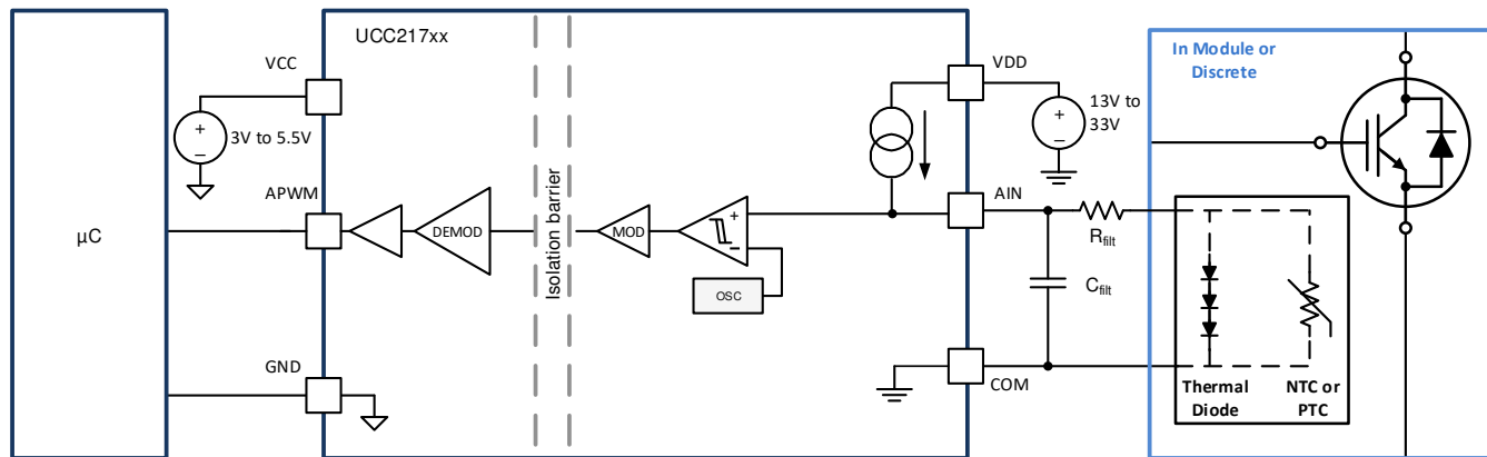
FIG 9-7. Thermal Diode or Thermistor Temperature Sensing Configuration
