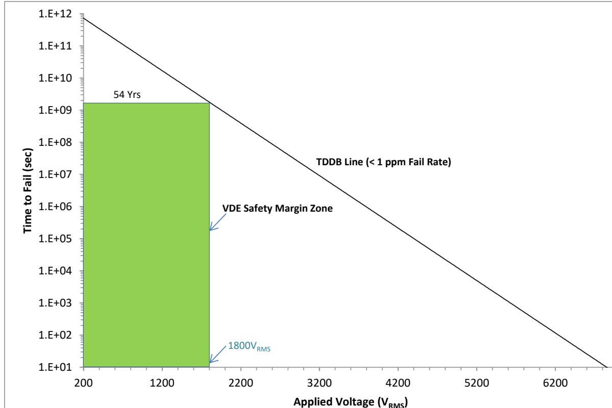
Figure 6-1. Reinforced Isolation Capacitor Life Time Projection
