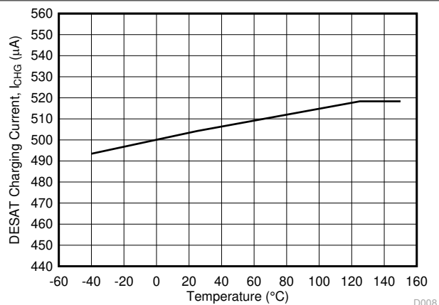
FIG 6-29. I_{\text{CHG}} DESAT Charging Current vs Temperature
