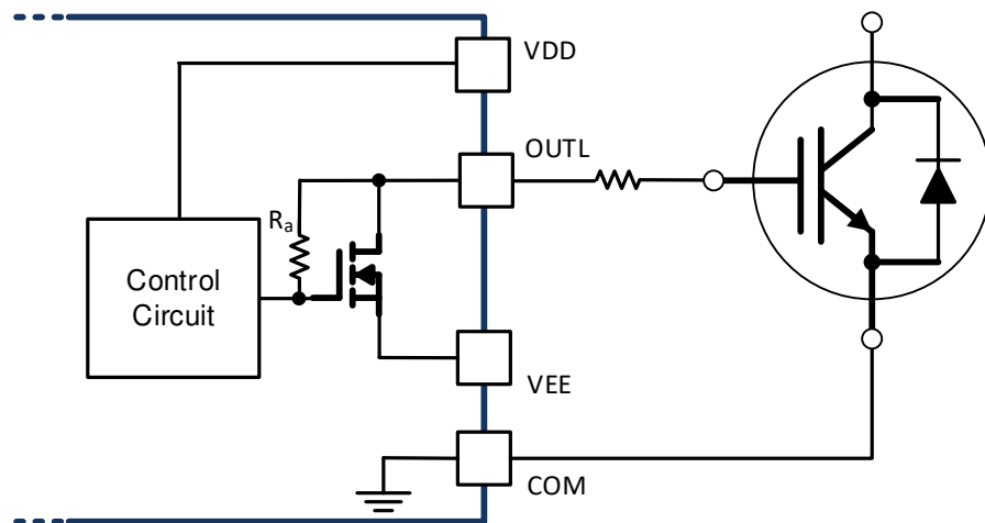
8-2. Active Pulldown
