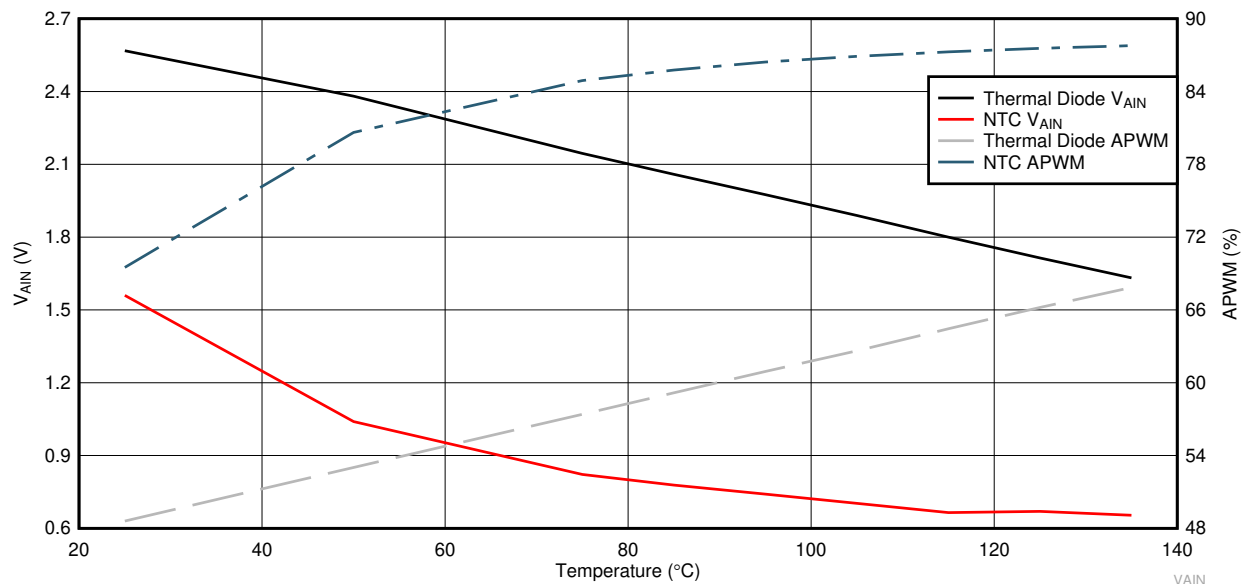
図 9-9. Thermal Diode and NTC V_{AIN} and Corresponding Duty Cycle at APWM
