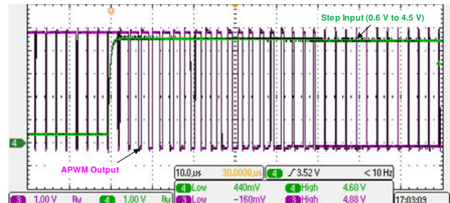
9-15. AIN Step Input (Green) and APWM Output (Pink)
