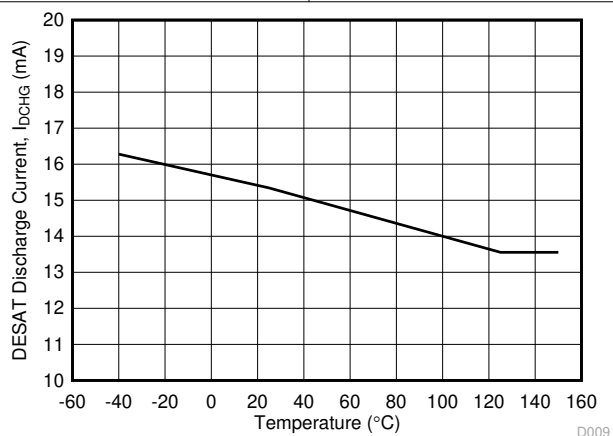
FIG 6-30. I_{\text{DCHG}} DESAT Discharge Current vs Temperature
