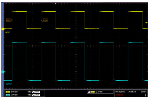
9-14. PWM Input (Yellow) and Driver Output (Blue)
