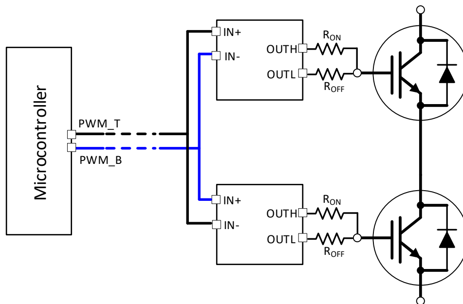
図 9-2. PWM Interlock for a Half Bridge
